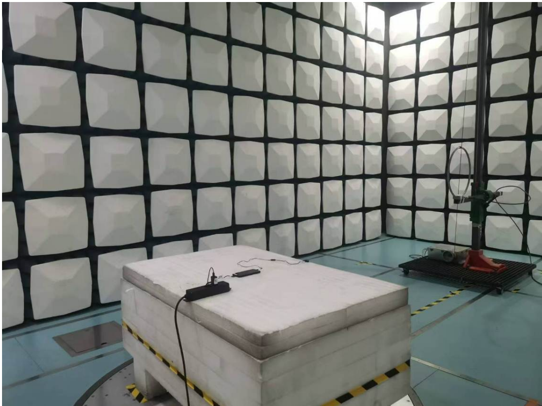
Radiated Emission 9k-30MHz Perpendicular View-128G
