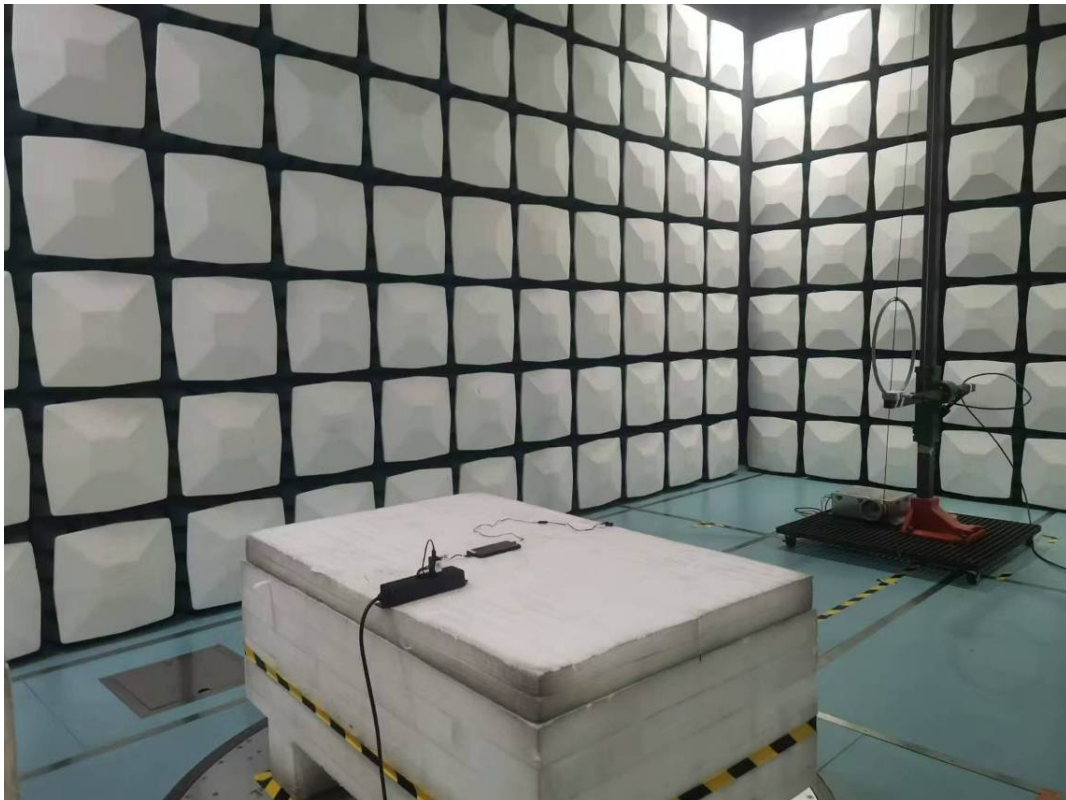
Radiated Emission 9k-30MHz Perpendicular View-64G
