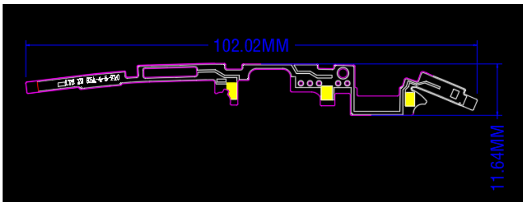
Dimensional drawing of GPS/WIFI/BT antenna
