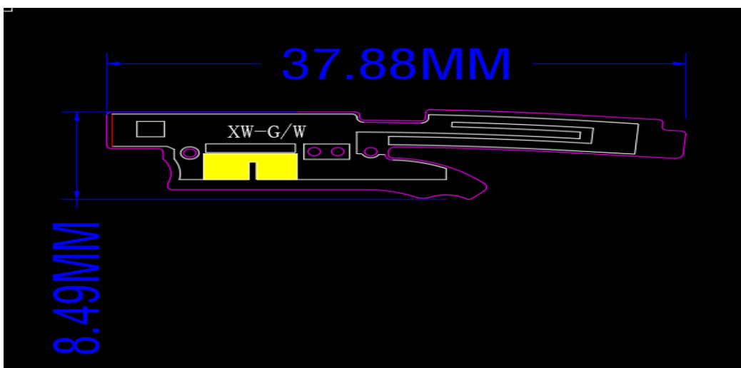
Dimensional drawing of diversity antenna
