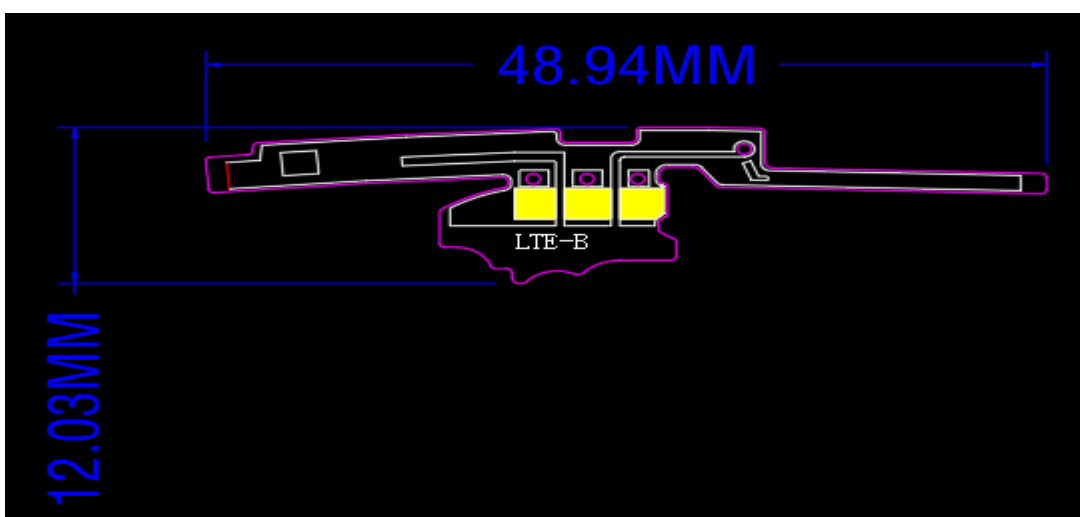
Dimensional drawing of diversity antenna
