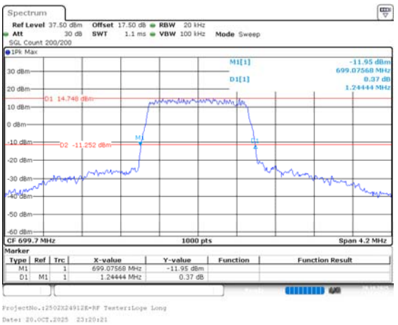
26dB Bandwidth
