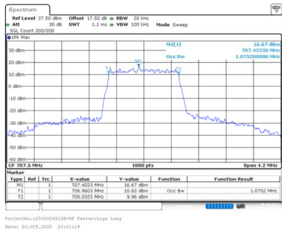
Occupied Bandwidth
