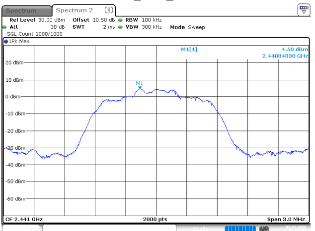
3EDR_DH1_Middle
