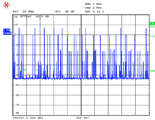
BDR_DH5_Hopping
