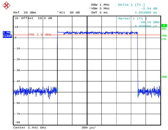
3EDR_DH3_Hopping
