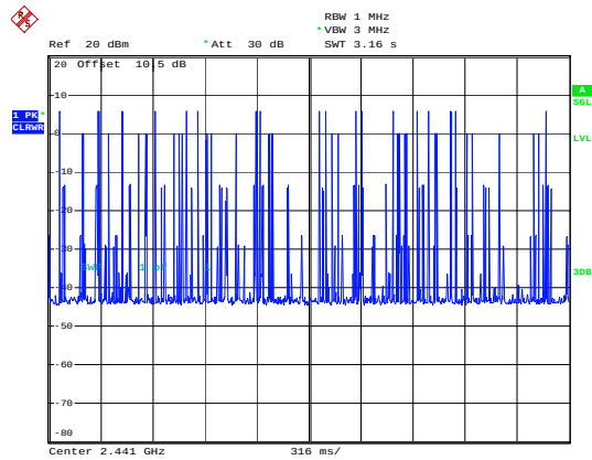
3EDR_DH3_Hopping
