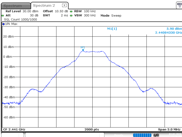
BDR_DH1_Middle
