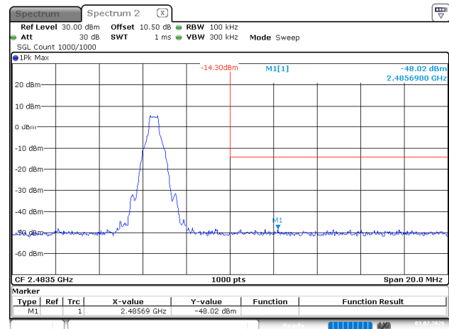
BDR_DH1_High
