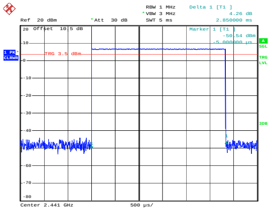
BDR_DH5_Hopping
