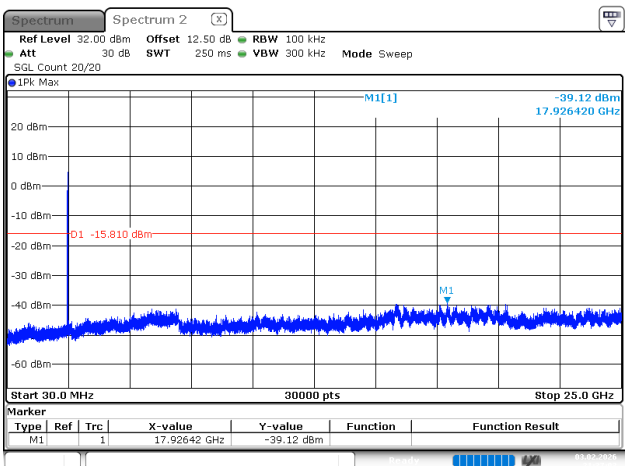
3EDR_DH1_High
