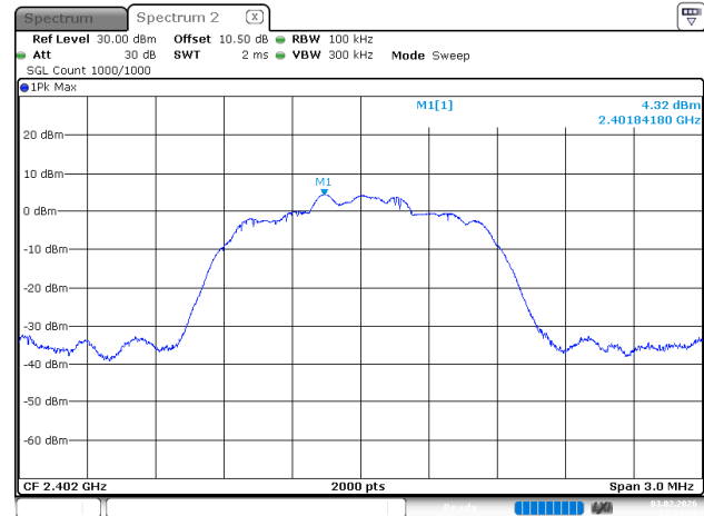
3EDR_DH1_Low
