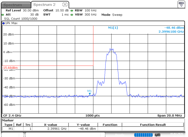
3EDR_DH1_Low
