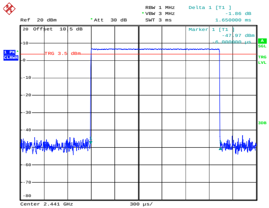
BDR_DH3_Hopping
