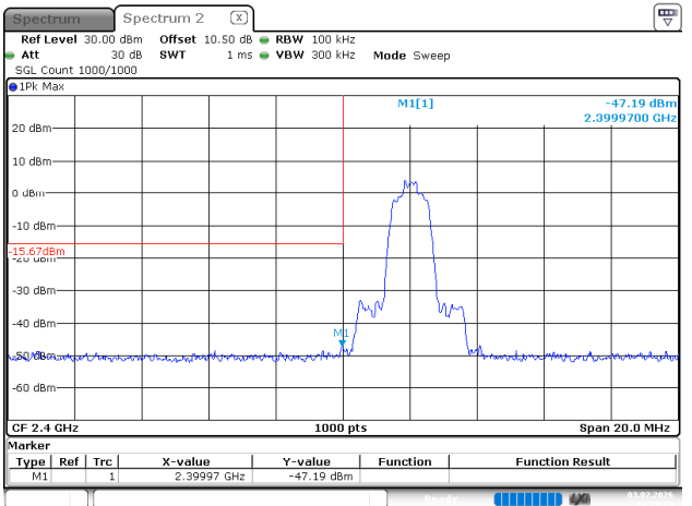
2EDR_DH1_Low
