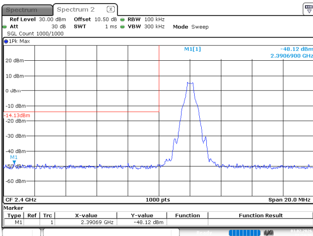
BDR_DH1_Low
