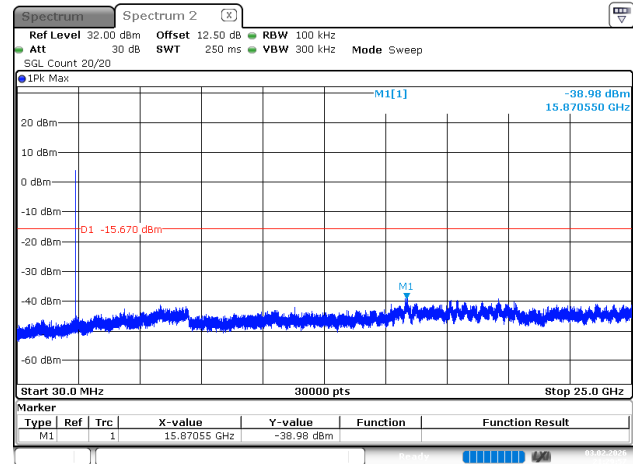
2EDR_DH1_Low
