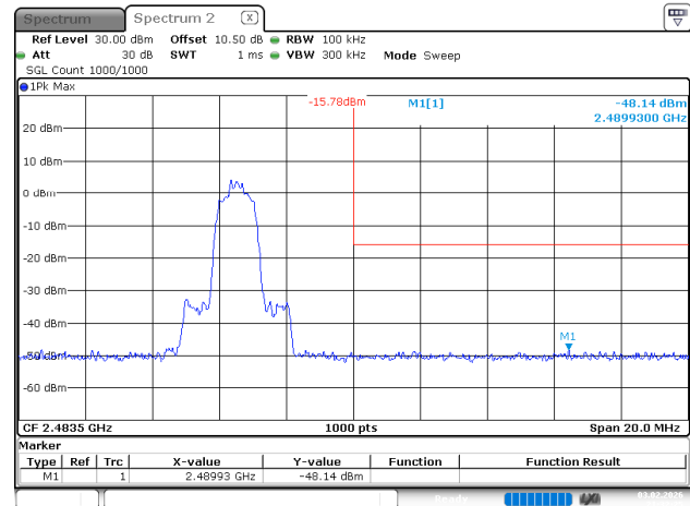
2EDR_DH1_High
