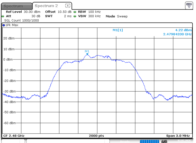
2EDR_DH1_High
