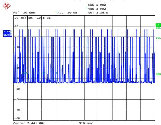
BDR_DH1_Hopping
