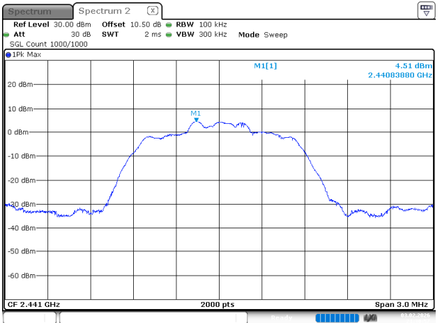
2EDR_DH1_Middle
