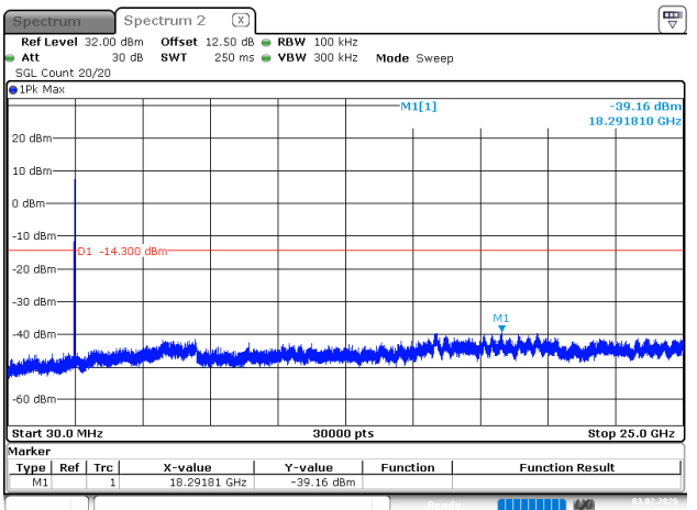
BDR_DH1_High
