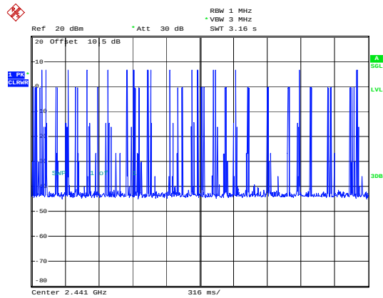
BDR_DH3_Hopping
