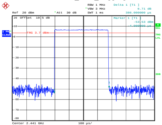
BDR_DH1_Hopping
