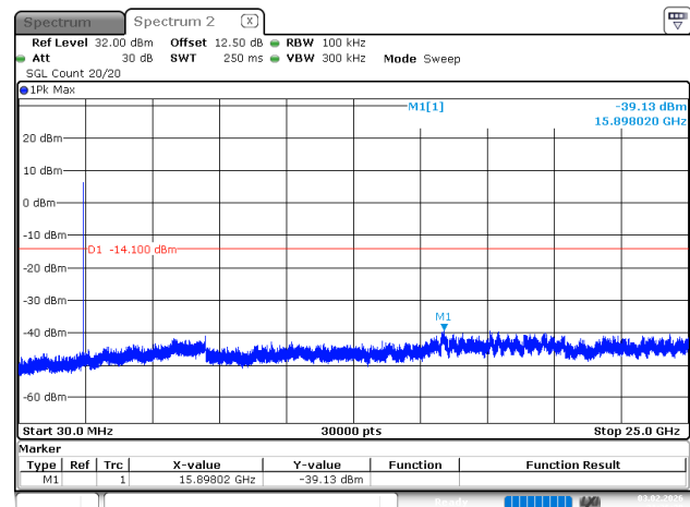
BDR_DH1_Middle
