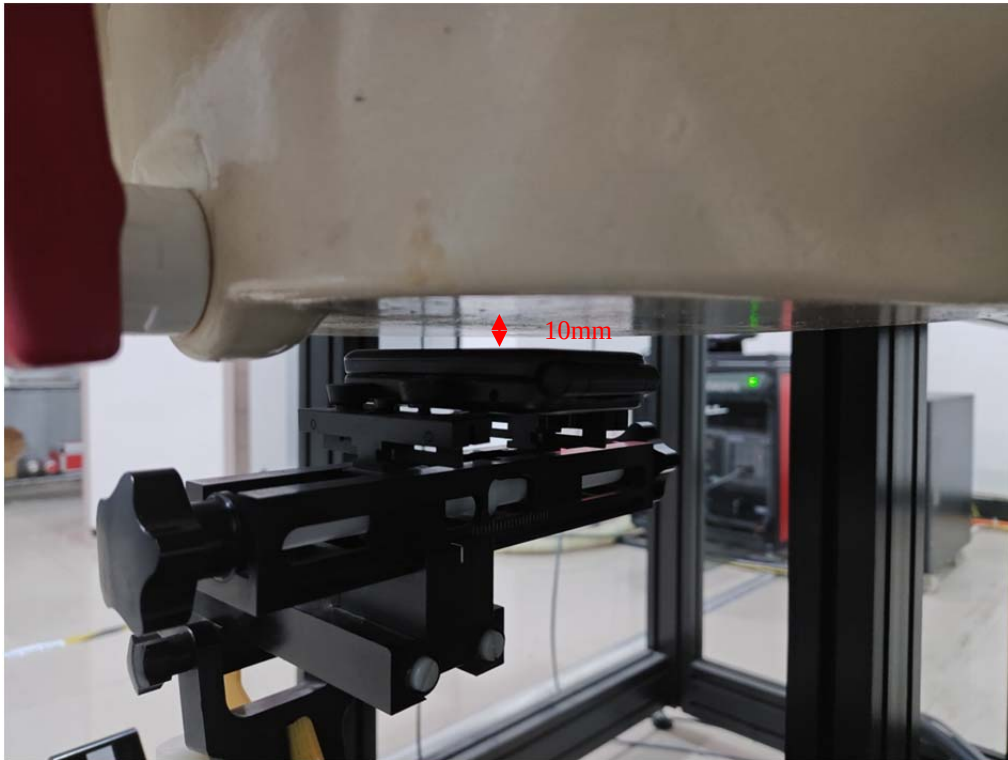
Body Back Fold Setup Photo (10mm)
