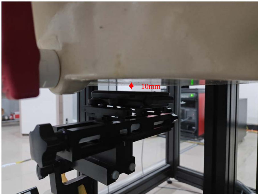
Body Back Fold Setup Photo (10mm)
