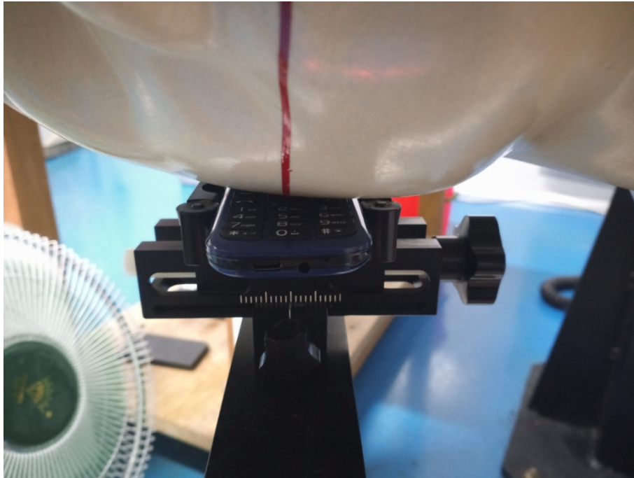
Head Right Cheek Setup Photo(0mm)
