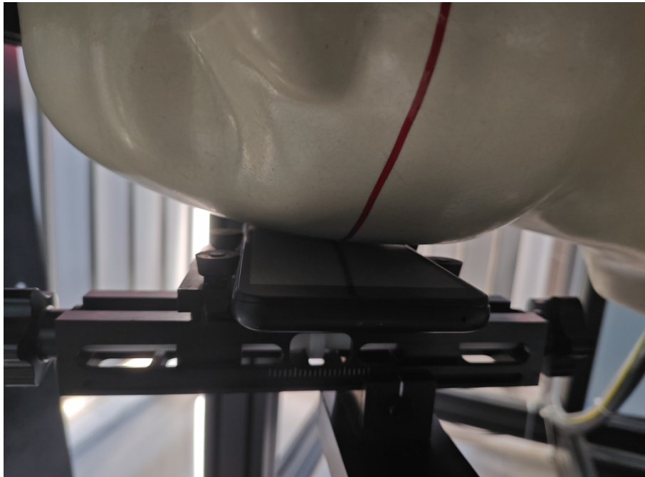
Head Right Cheek Setup Photo (0mm)
