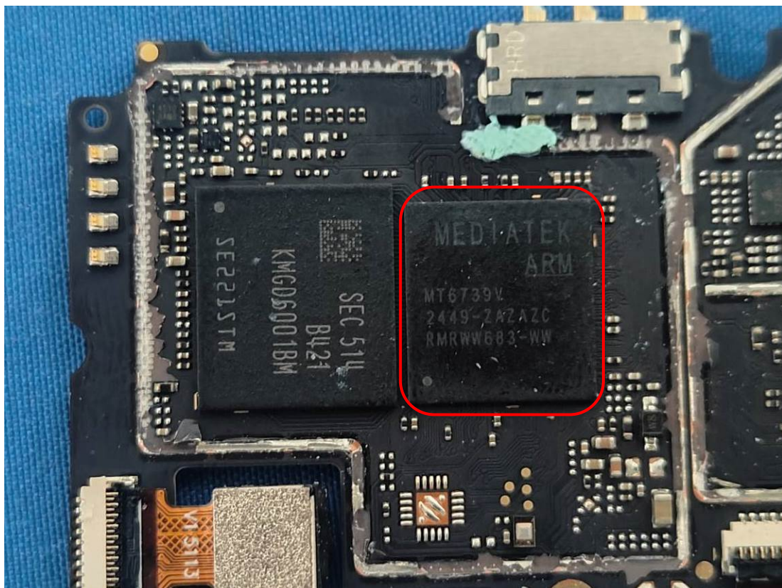
Main Chip
