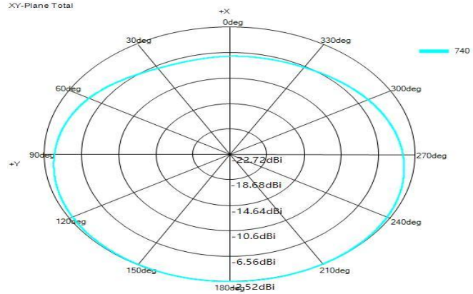
XY-Plane Total
