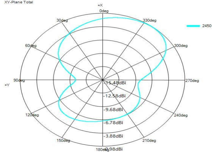
XY-Plane Total
