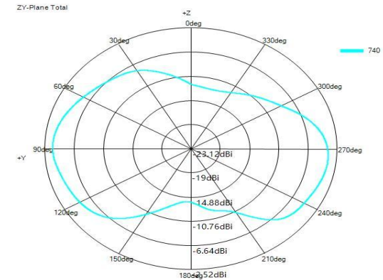
ZY-Plane Total
