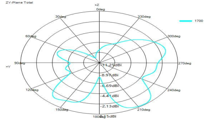
ZY-Plane Total
