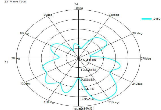
ZY-Plane Total
