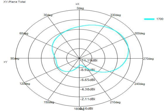
XY-Plane Total
