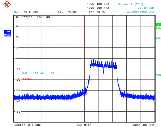
802.11g_2412MHz
