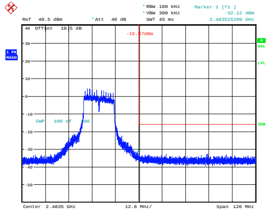
802.11g_2462MHz
