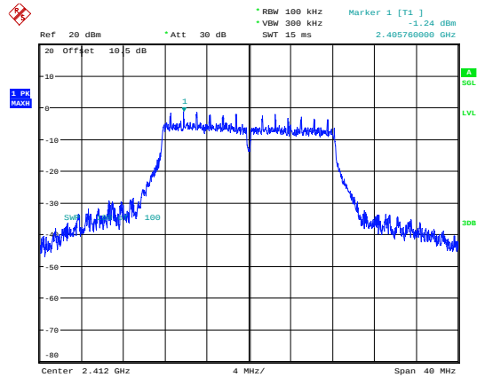
802.11g_2412MHz
