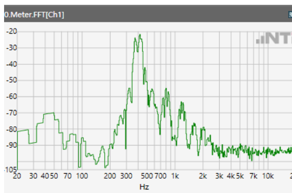
ANSI/TIA 5050-2018 \ 8N HAC OFF \ NB 12.2kbps\ 5.2 Receive path – distortion and noise\LTE Band 5
