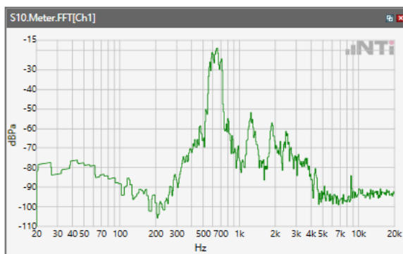
ANSI/TIA 5050-2018 \ 2N HAC ON \ NB 12.2kbps\ 5.2 Receive path – distortion and noise\LTE Band 17
