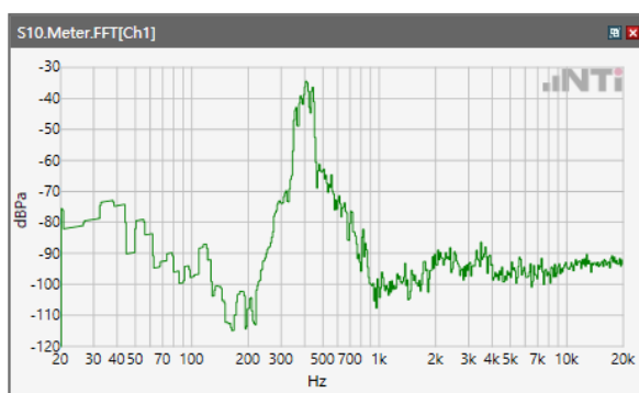
ANSI/TIA 5050-2018 \ 2N HAC ON \ NB 12.2kbps\ 5.2 Receive path – distortion and noise\WCDMA Band V
