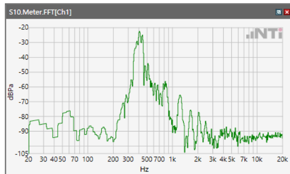
ANSI/TIA 5050-2018 \ 2N HAC ON \ NB 12.2kbps\ 5.2 Receive path – distortion and noise\LTE Band 2
