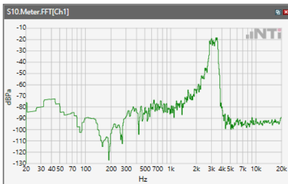
ANSI/TIA 5050-2018 \ 2N HAC ON \ NB 12.2kbps\ 5.2 Receive path – distortion and noise\LTE Band 7
