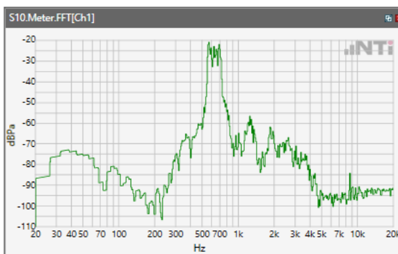
ANSI/TIA 5050-2018 \ 2N HAC ON \ NB 12.2kbps\ 5.2 Receive path – distortion and noise\LTE Band 66
