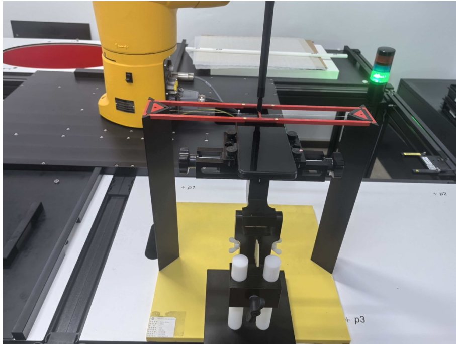
Test Setup Photos 1.
