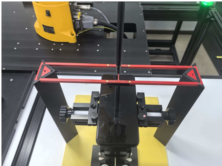
Test Setup Photos 2.
