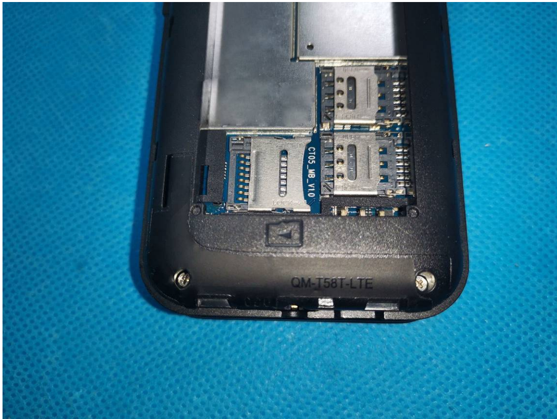
Aux Antenna
