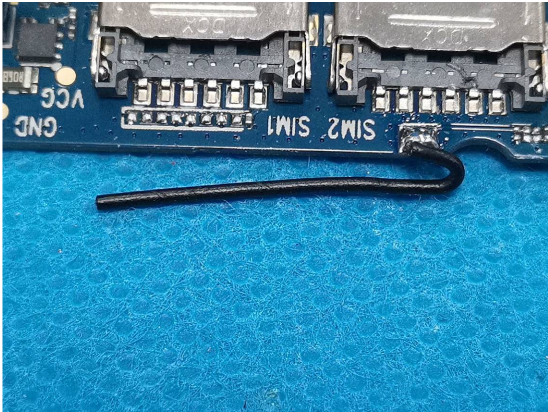
Bluetooth Antenna
