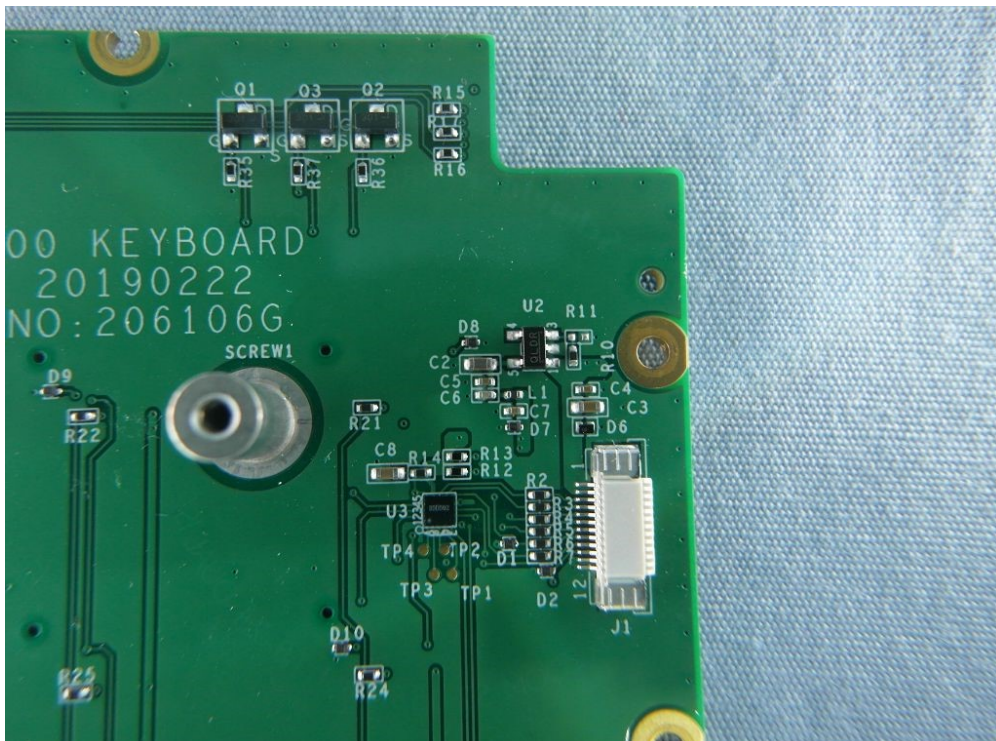
(22) EUT Photo
