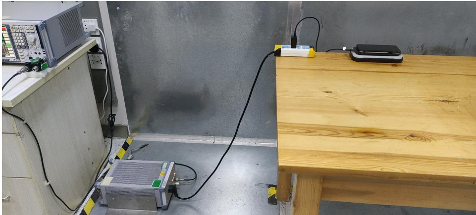
Photo of Conducted Emission Measurement FCC ID: 2ASPB-CELL
