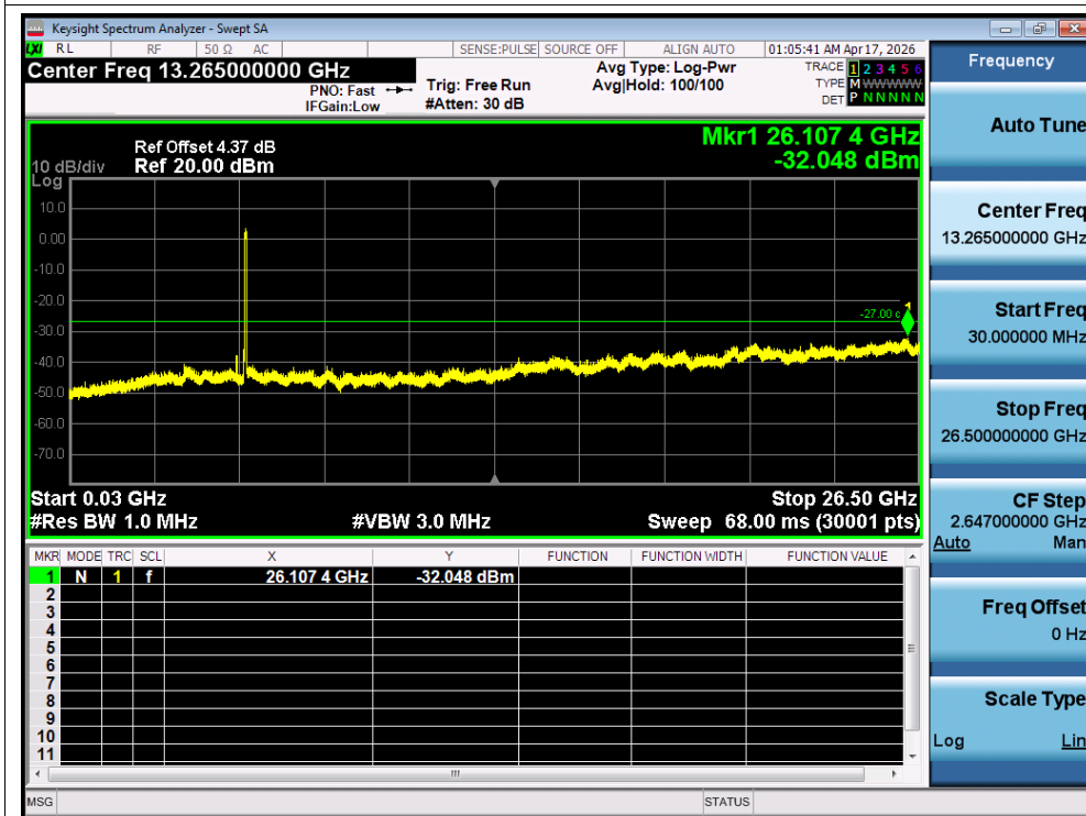
Tx. Spurious NVNT ax40 5550MHz Ant B Emission
