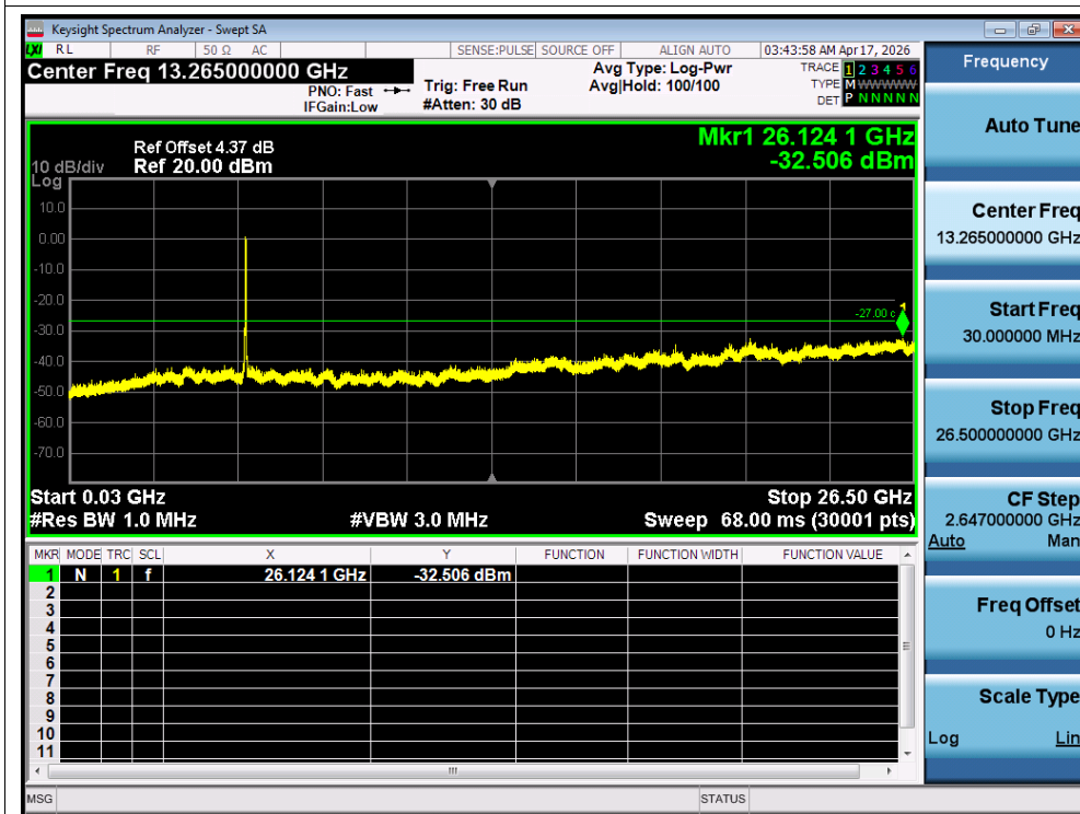
Tx. Spurious NVNT n40 5550MHz Ant A Emission
