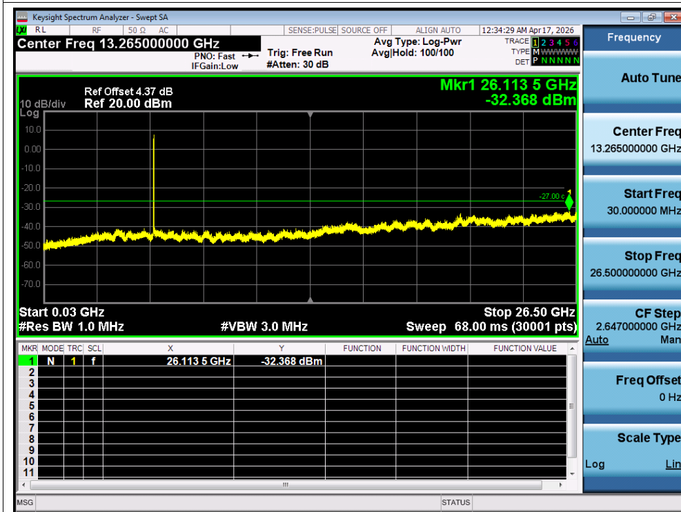
Tx. Spurious NVNT n20 5500MHz Ant B Emission
