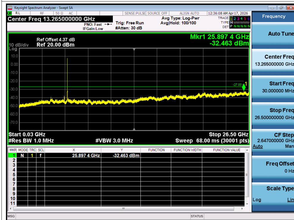
Tx. Spurious NVNT n20 5700MHz Ant B Emission
