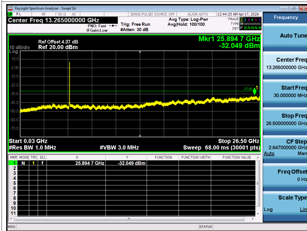
Tx. Spurious NVNT ax20 5500MHz Ant B Emission
