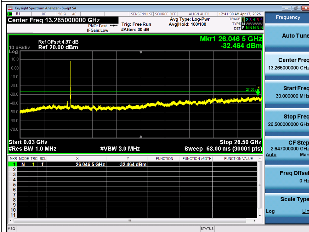
Tx. Spurious NVNT ac20 5700MHz Ant B Emission
