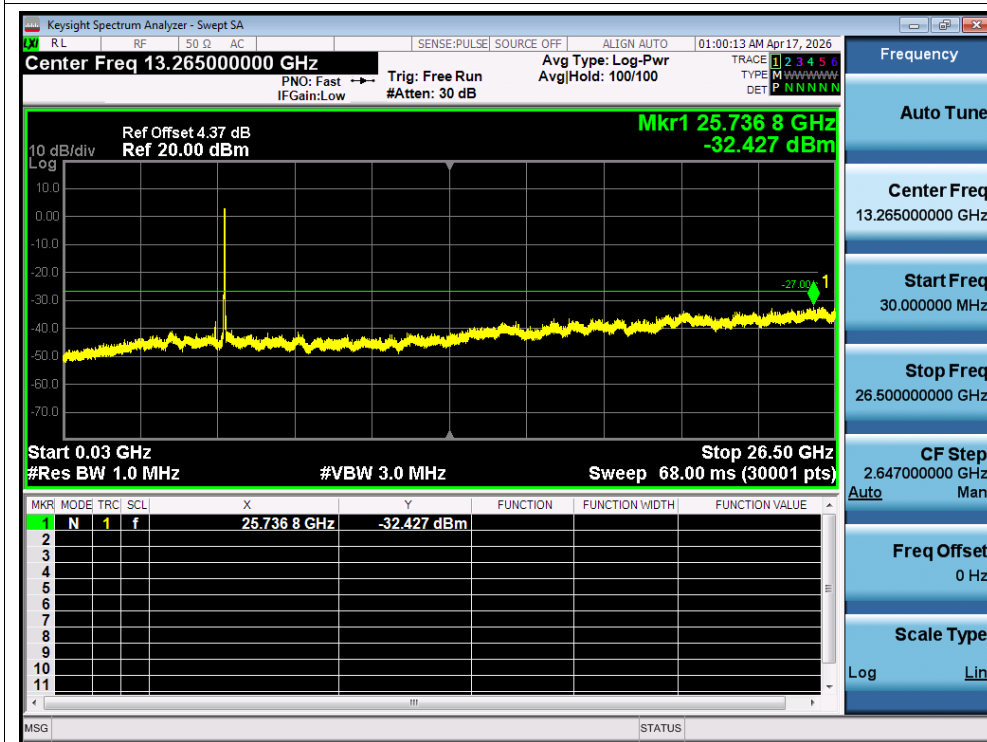
Tx. Spurious NVNT ac40 5550MHz Ant B Emission
