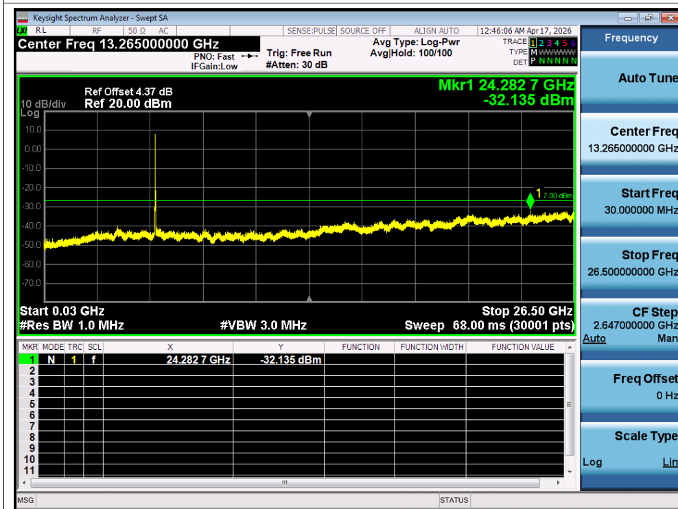
Tx. Spurious NVNT ax20 5700MHz Ant B Emission
