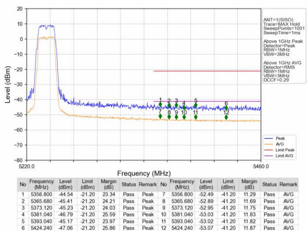
802.11a_LCH_5260MHz_Ant1_NTNV
