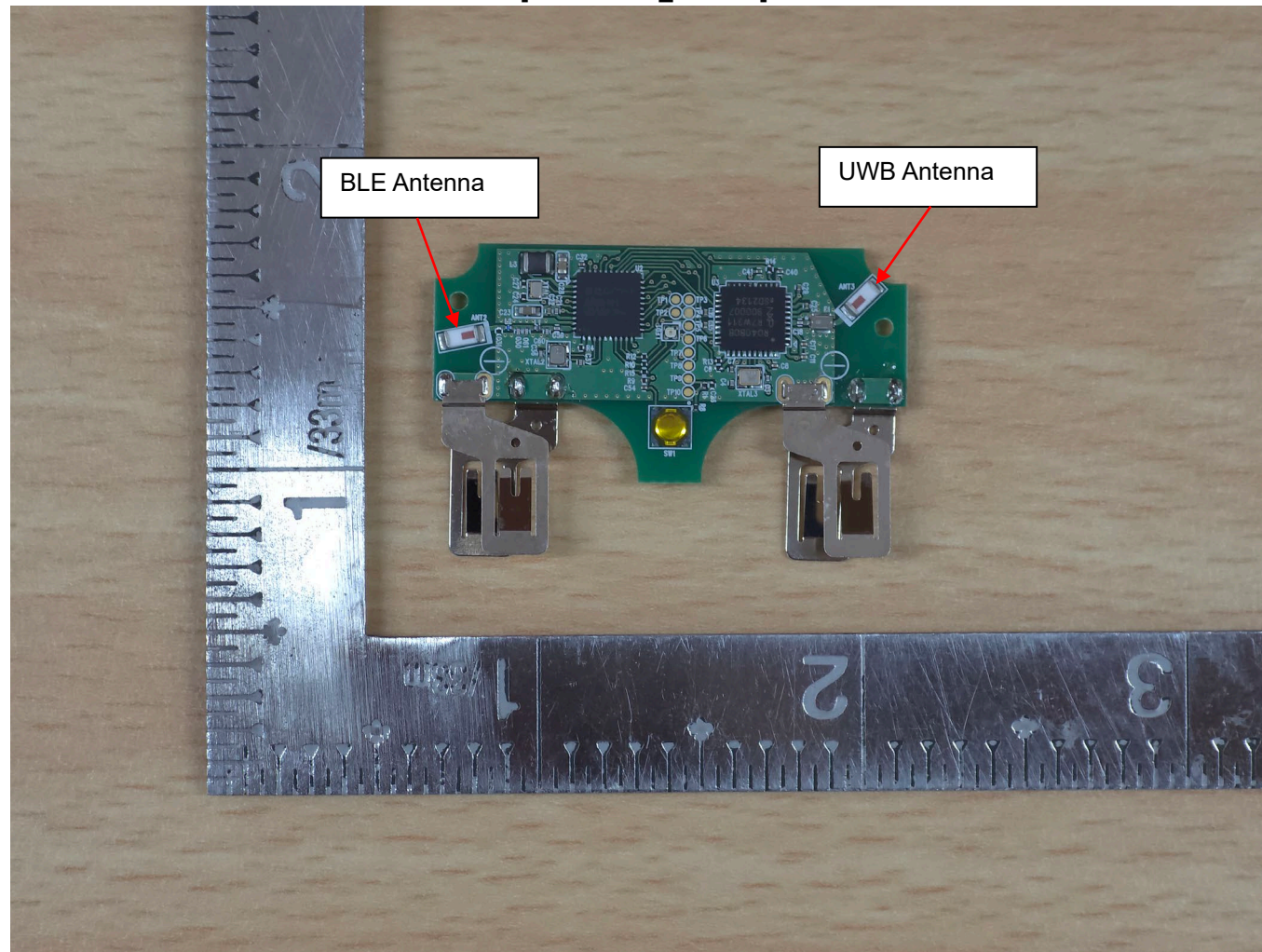
[PCB Board_Bottom]
