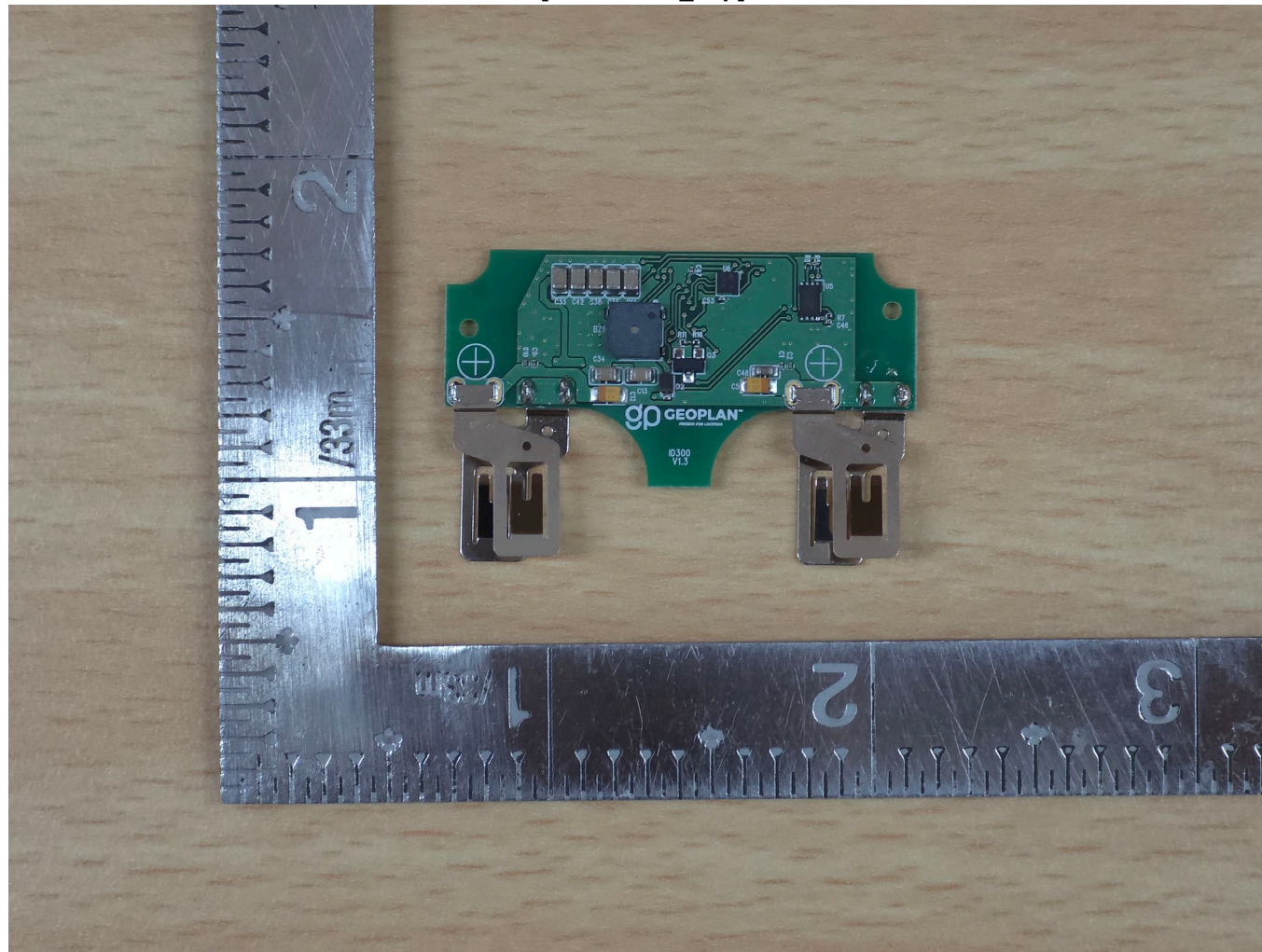
[PCB Board_Top]
