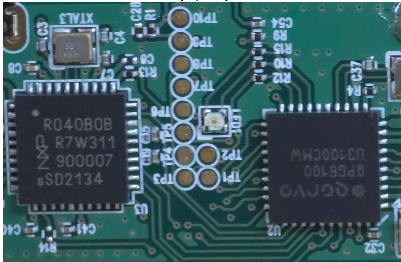
[Chip Photo]
