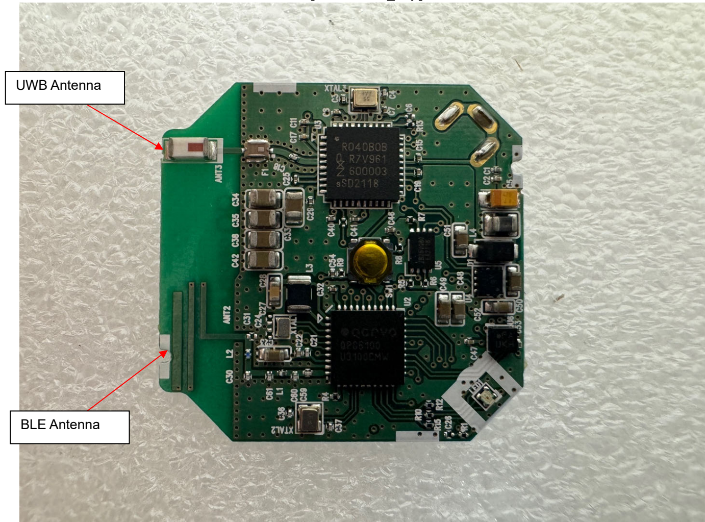
[Main board_Top]
