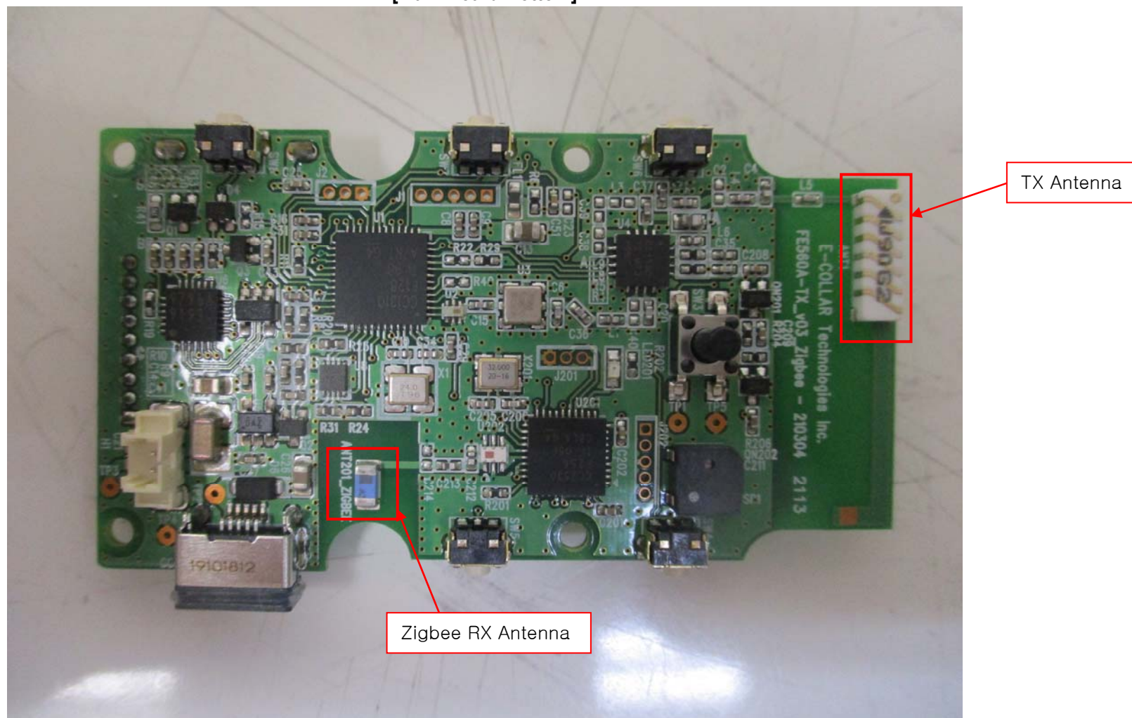
[Main Board Bottom]
