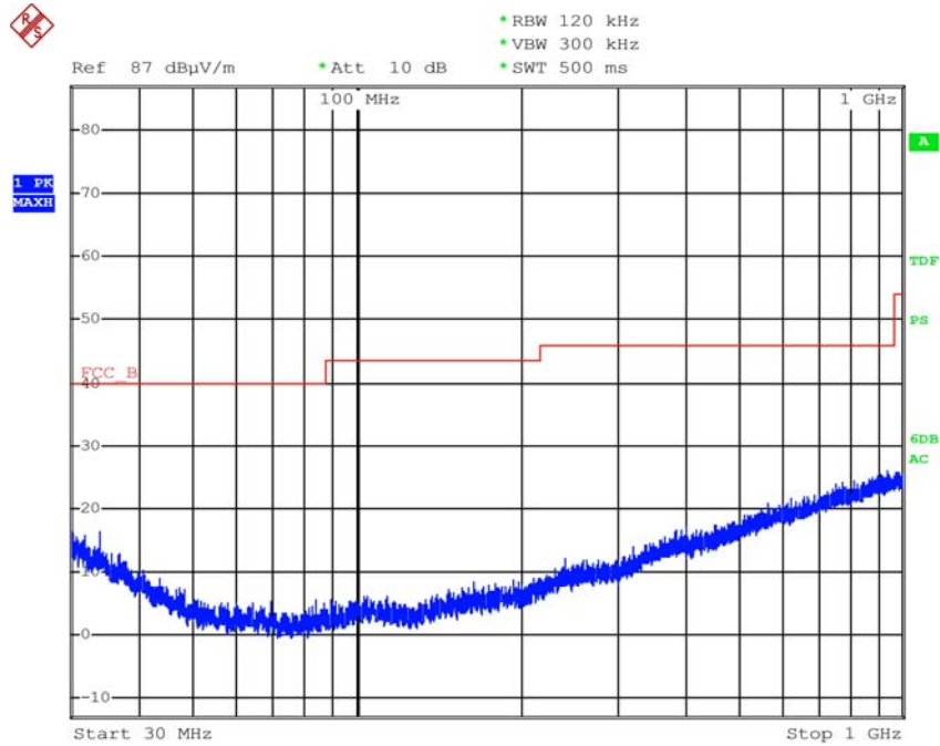
Radiated emissions (Below 1 000 MHz)
