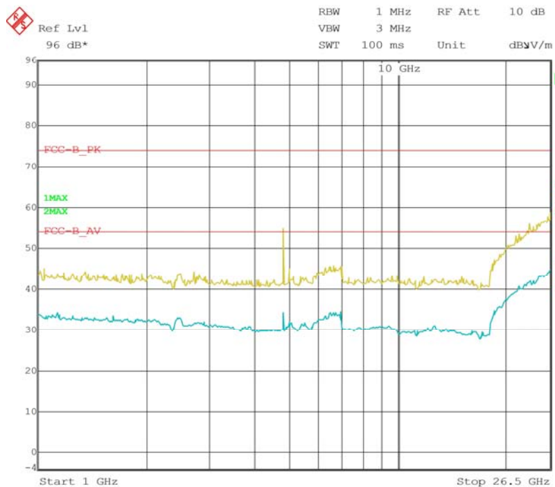
Radiated emissions (Above 1 000 MHz)
