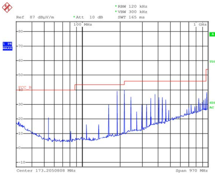
Radiated emissions (Below 1 000 MHz)
