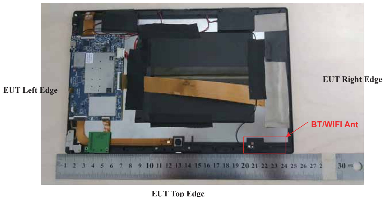
Back View
