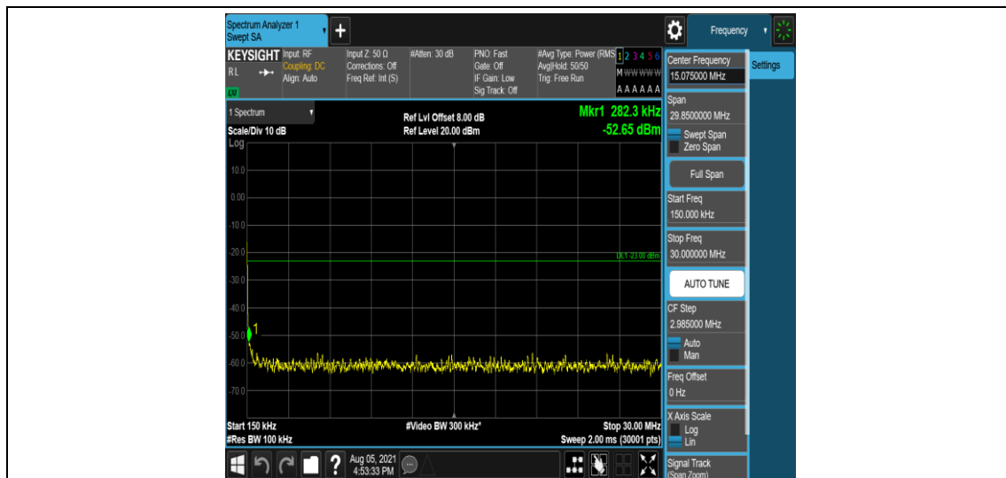
Band12-1.4MHz-QPSK-23173-1-0-High-0.15-30--52.66-PASS
