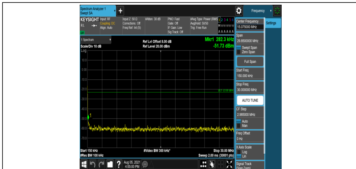
Band12-1.4MHz-16QAM-23173-1-0-High-0.15-30--51.73-PASS
