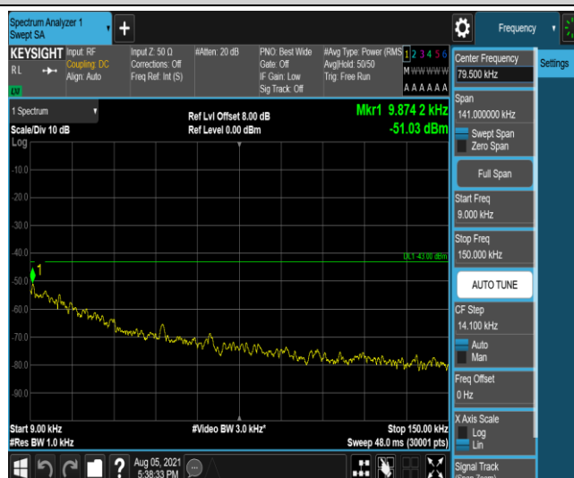
Band12-3MHz-QPSK-23095-1-0-Low-0.009-0.15--51.03-PASS
