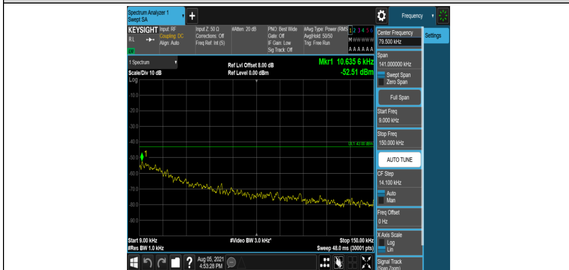
Band12-1.4MHz-QPSK-23173-1-0-High-0.009-0.15--52.51-PASS
