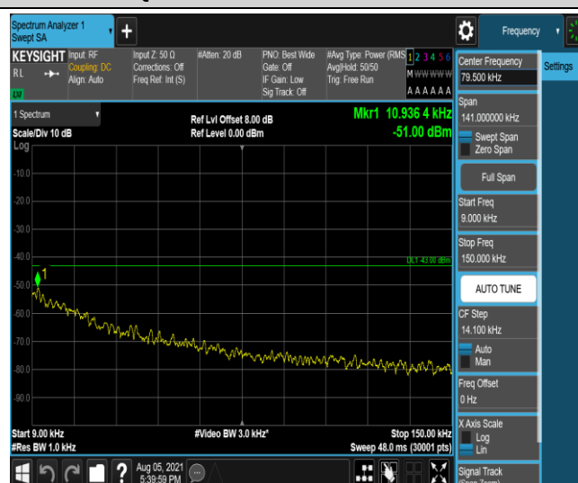
Band12-3MHz-16QAM-23095-1-0-Low-0.009-0.15--51-PASS
