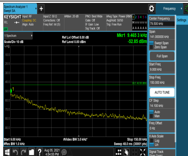
Band12-1.4MHz-16QAM-23173-1-0-High-0.009-0.15--52.85-PASS
