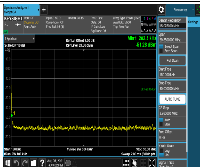
Band12-1.4MHz-16QAM-23017-1-0-Low-0.15-30--51.28-PASS
