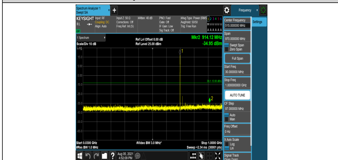
Band12-1.4MHz-16QAM-23095-1-0-Low-30-1000--34.96-PASS
