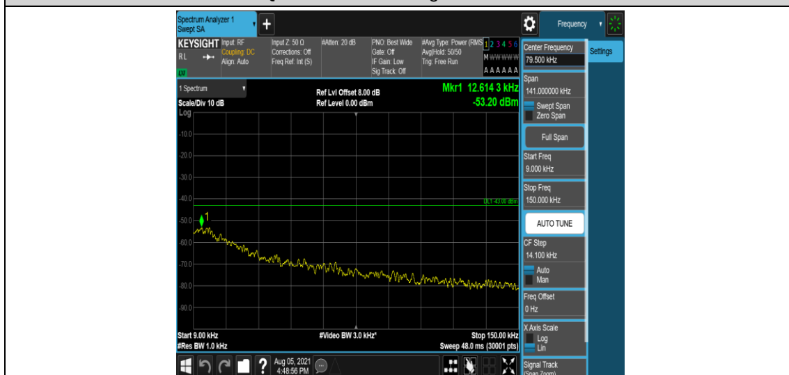
Band12-1.4MHz-16QAM-23017-1-0-Low-0.009-0.15--53.2-PASS
