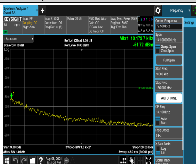
Band12-3MHz-QPSK-23165-1-0-High-0.009-0.15--51.73-PASS
