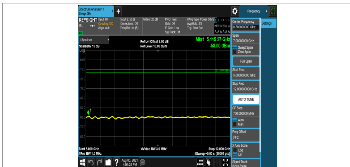
Band12-1.4MHz-QPSK-23173-1-0-High-5000-12000--58-PASS
