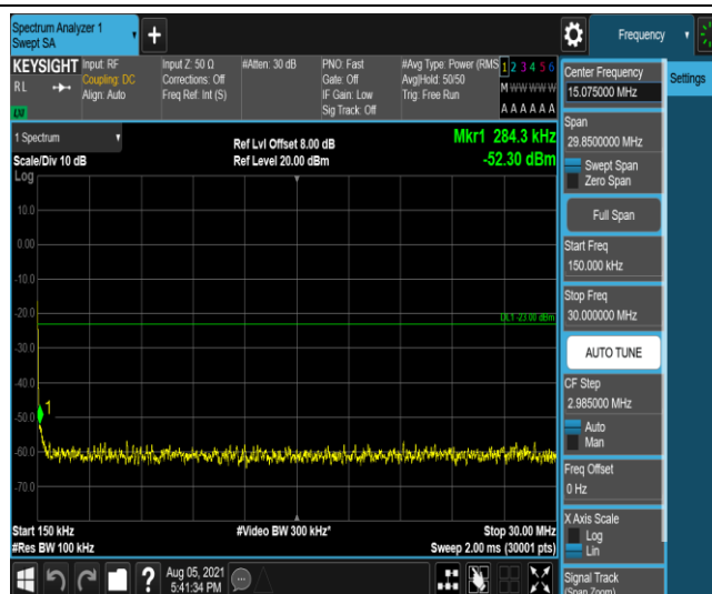
Band12-3MHz-QPSK-23165-1-0-High-0.15-30--52.3-PASS
