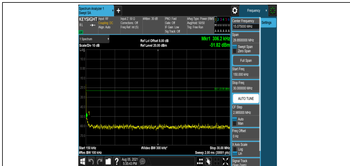
Band12-3MHz-QPSK-23025-1-0-Low-0.15-30--51.82-PASS
