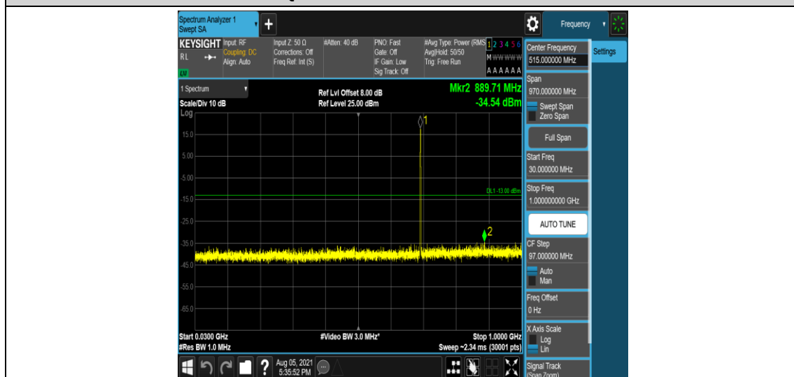
Band12-3MHz-QPSK-23025-1-0-Low-30-1000--34.54-PASS
