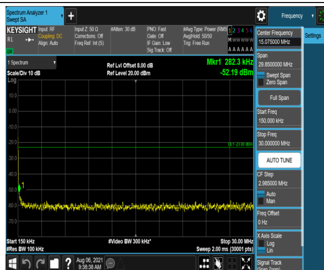
Band12-5MHz-16QAM-23155-1-0-High-0.15-30--52.19-PASS
