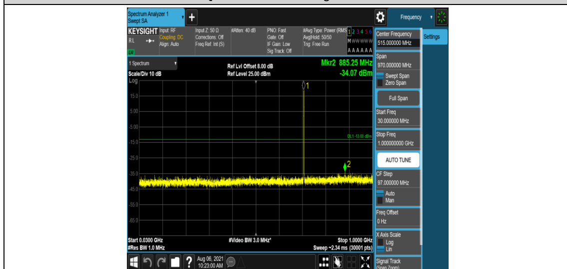
Band12-10MHz-QPSK-23130-1-0-High-30-1000--34.07-PASS
