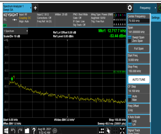
Band12-5MHz-16QAM-23035-1-0-Low-0.009-0.15--53.44-PASS
