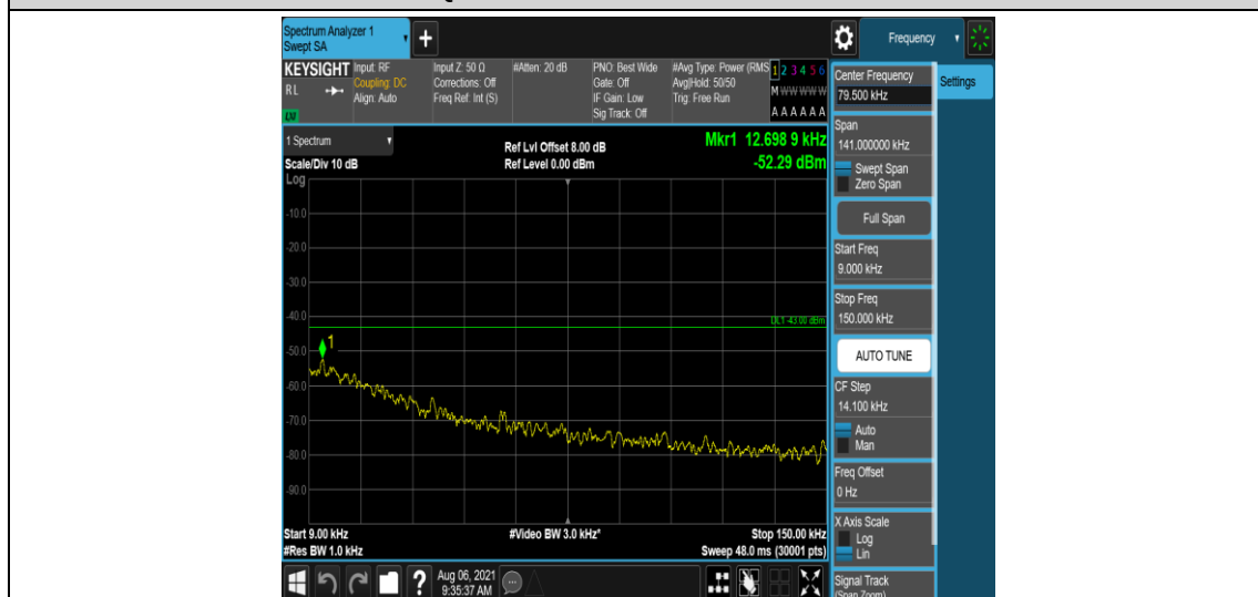
Band12-5MHz-16QAM-23095-1-0-Low-0.009-0.15--52.29-PASS
