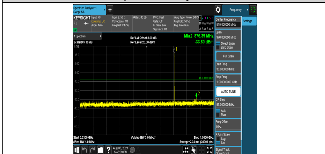
Band12-3MHz-16QAM-23165-1-0-High-30-1000--33.6-PASS
