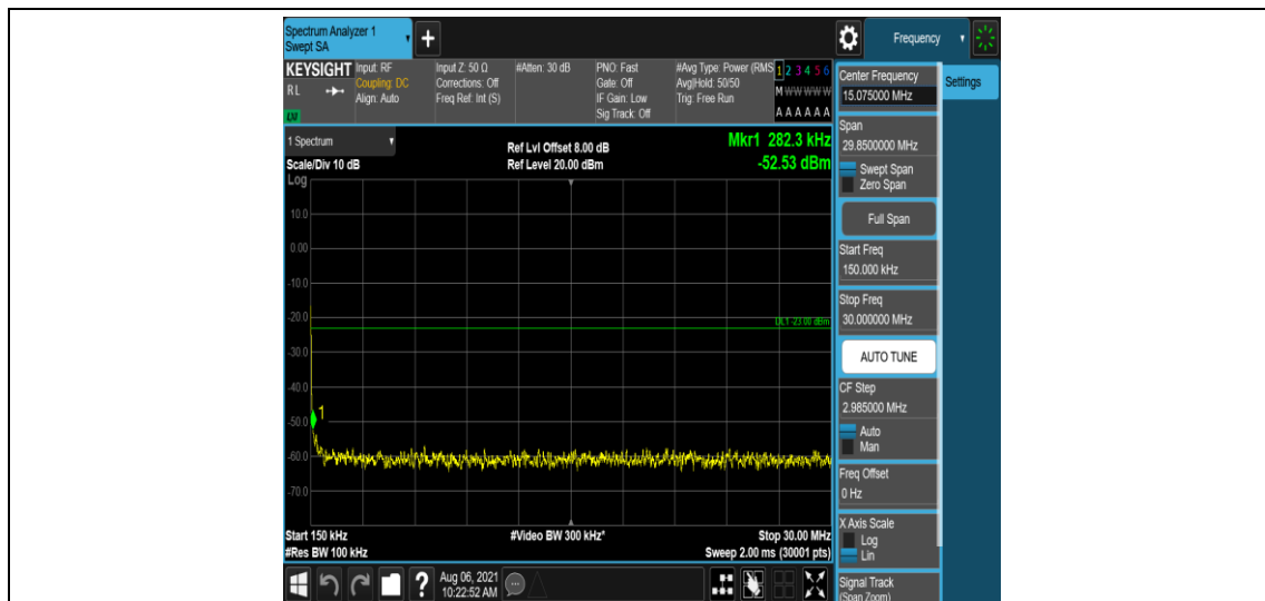
Band12-10MHz-QPSK-23130-1-0-High-0.15-30--52.54-PASS
