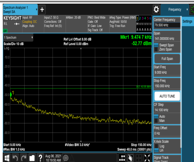
Band12-10MHz-QPSK-23095-1-0-Low-0.009-0.15--52.77-PASS
