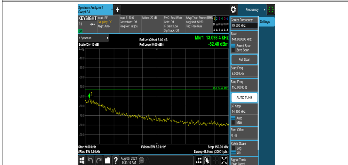
Band12-5MHz-QPSK-23035-1-0-Low-0.009-0.15--52.48-PASS
