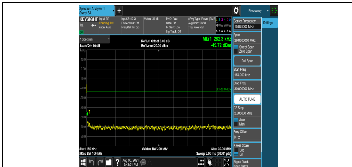
Band12-3MHz-16QAM-23165-1-0-High-0.15-30--49.72-PASS
