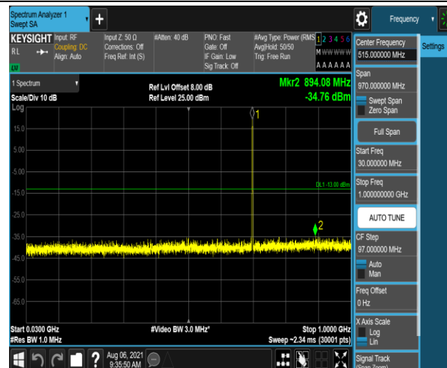
Band12-5MHz-16QAM-23095-1-0-Low-30-1000--34.77-PASS
