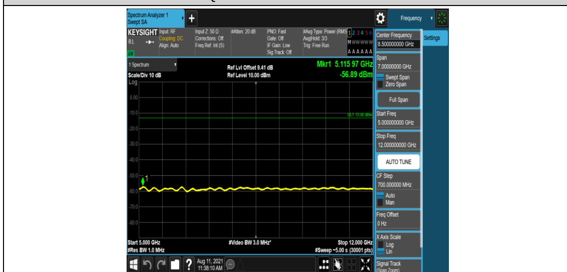
Band25-20MHz-16QAM-26140-1-0-Low-5000-12000--56.89-PASS
