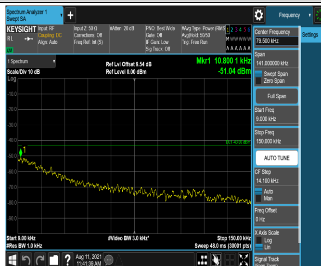
Band25-20MHz-QPSK-26590-1-0-High-0.009-0.15--51.04-PASS
