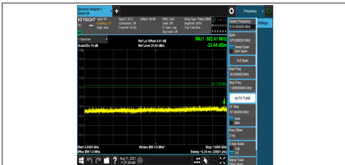
Band25-20MHz-16QAM-26140-1-0-Low-30-1000--33.44-PASS
