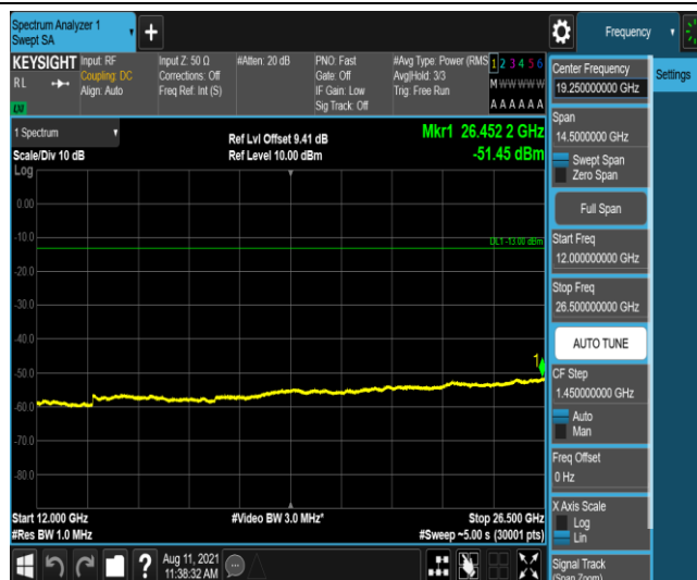
Band25-20MHz-16QAM-26140-1-0-Low-12000-26500--51.45-PASS
