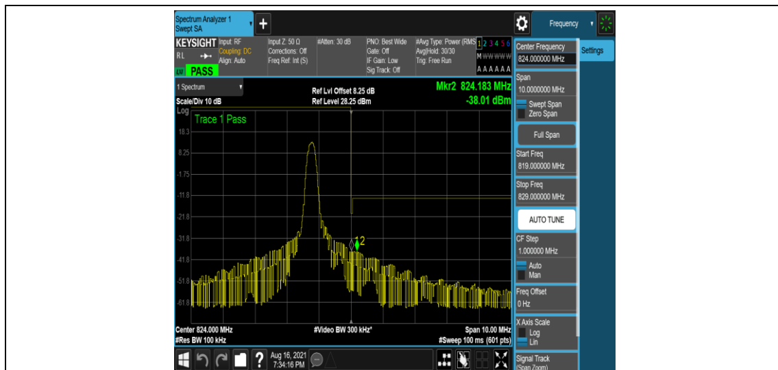
Band26-5MHz-QPSK-26765-1-0-High--37.98,-38.01-PASS
