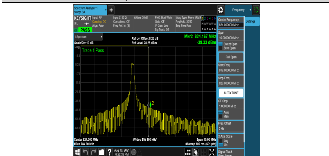
Band26-1.4MHz-QPSK-26783-1-0-High--39.71,-39.33-PASS
