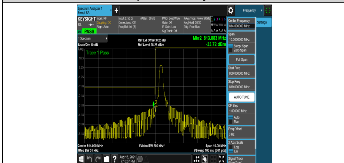
Band26-3MHz-QPSK-26705-1-0-Low--36.47,-33.72-PASS
