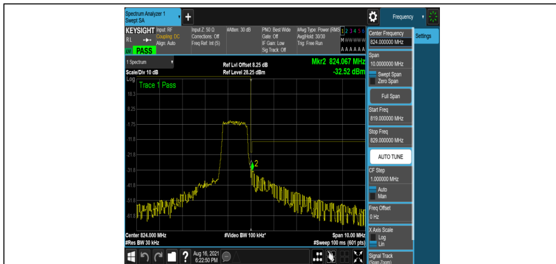
Band26-1.4MHz-QPSK-26783-6-0-High--31.22,-32.52-PASS
