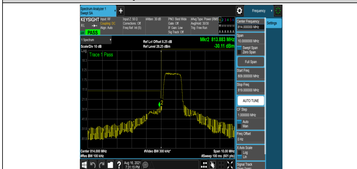
Band26-5MHz-QPSK-26715-6-0-Low--28.36,-30.11-PASS
