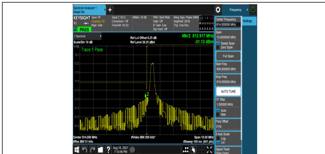
Band26-3MHz-16QAM-26705-1-0-Low--29.83,-31.13-PASS
