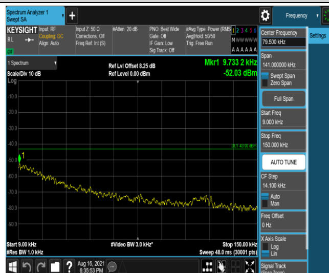
Band26-1.4MHz-QPSK-26783-1-0-High-0.009-0.15--52.03-PASS
