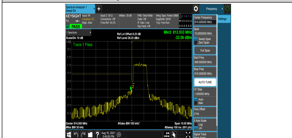
Band26-1.4MHz-16QAM-26697-6-0-Low--31.06,-33.56-PASS
