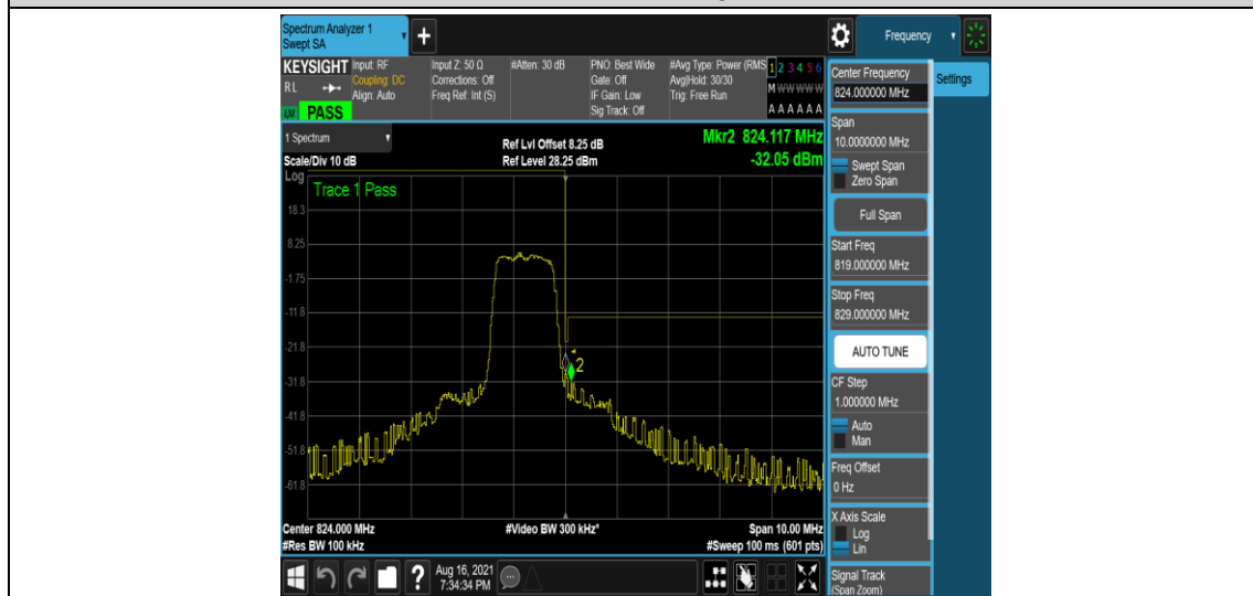
Band26-5MHz-QPSK-26765-6-0-High--29.36,-32.05-PASS
