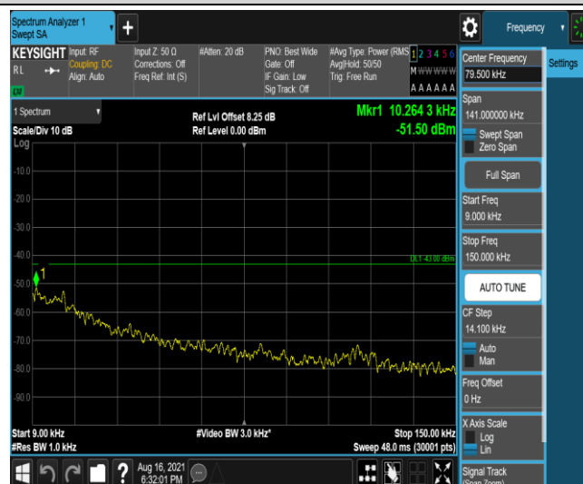
Band26-1.4MHz-QPSK-26740-1-0-Low-0.009-0.15--51.5-PASS
