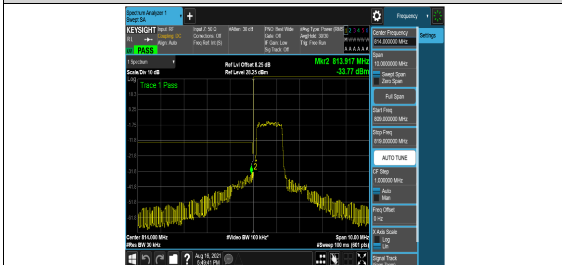
Band26-1.4MHz-QPSK-26697-6-0-Low--31.40,-33.77-PASS
