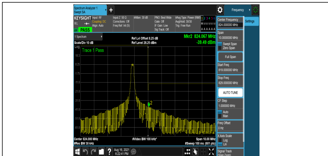
Band26-1.4MHz-16QAM-26783-1-0-High--39.34,-39.49-PASS
