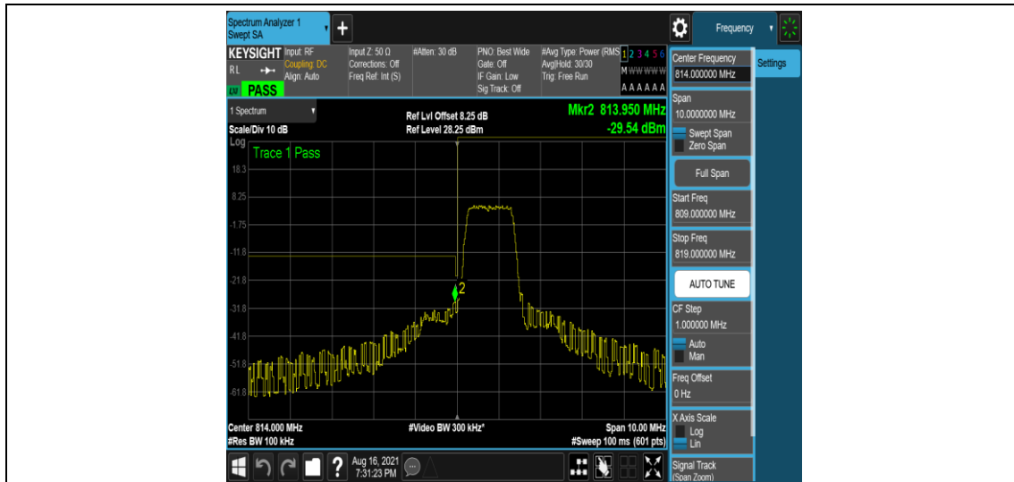
Band26-5MHz-16QAM-26715-6-0-Low--29.15,-29.54-PASS
