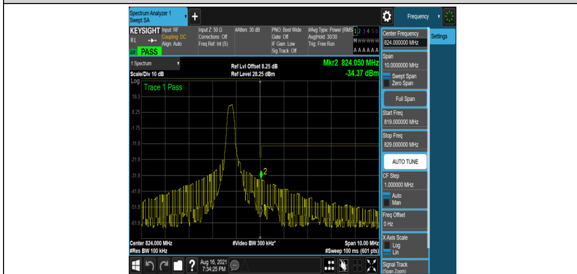
Band26-5MHz-16QAM-26765-1-0-High--57.13,-34.37-PASS
