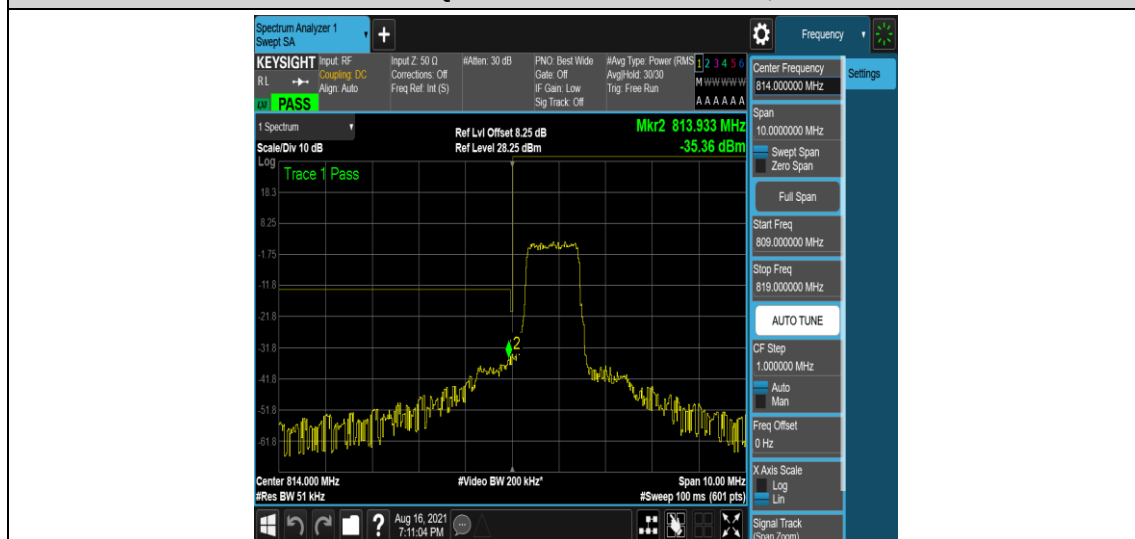
Band26-3MHz-16QAM-26705-6-0-Low--33.84,-35.36-PASS
