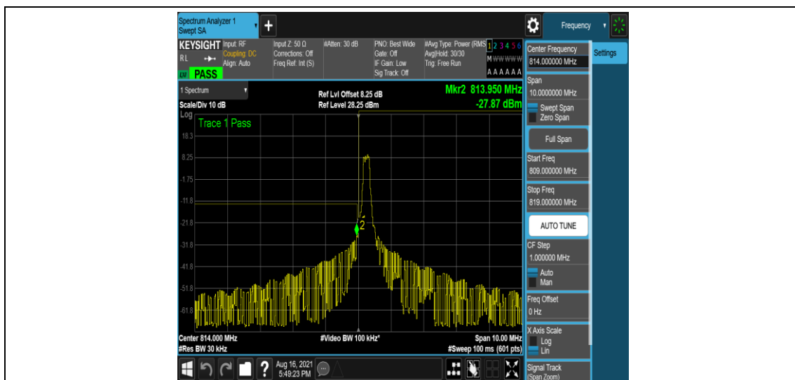
Band26-1.4MHz-QPSK-26697-1-0-Low--25.52,-27.87-PASS
