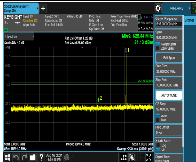
Band26-1.4MHz-16QAM-26697-1-0-Low-30-1000--34.13-PASS
