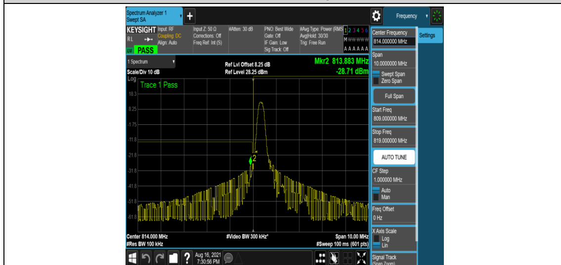
Band26-5MHz-QPSK-26715-1-0-Low--25.84,-28.71-PASS
