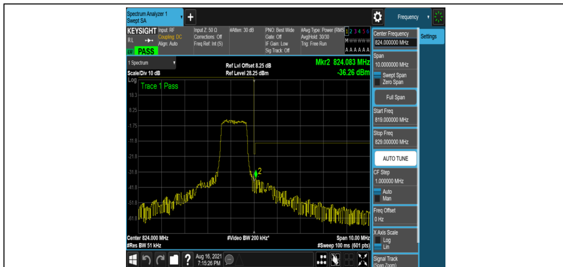
Band26-3MHz-16QAM-26775-6-0-High--38.31,-36.26-PASS
