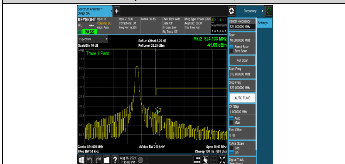
Band26-3MHz-16QAM-26775-1-0-High--39.44,-41.09-PASS
