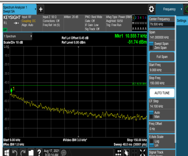
Band26-5MHz-QPSK-27015-1-0-High-0.009-0.15--51.75-PASS
