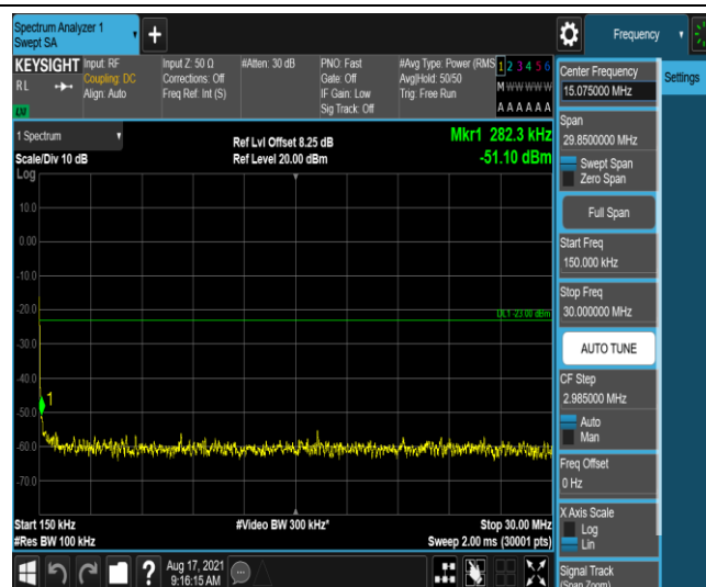
Band26-3MHz-16QAM-26805-1-0-Low-0.15-30--51.11-PASS
