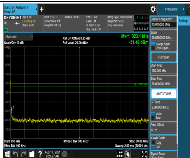
Band26-5MHz-QPSK-26815-1-0-Low-0.15-30--51.48-PASS
