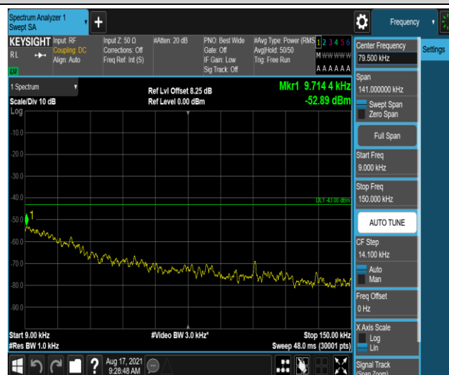
Band26-5MHz-16QAM-26815-1-0-Low-0.009-0.15--52.89-PASS
