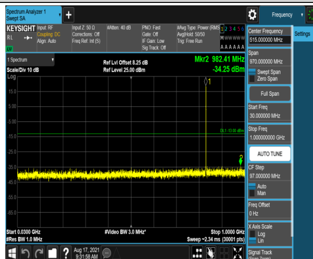
Band26-5MHz-16QAM-26915-1-0-Low-30-1000--34.25-PASS
