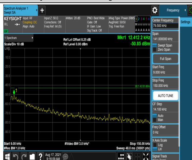
Band26-3MHz-16QAM-26805-1-0-Low-0.009-0.15--50.85-PASS
