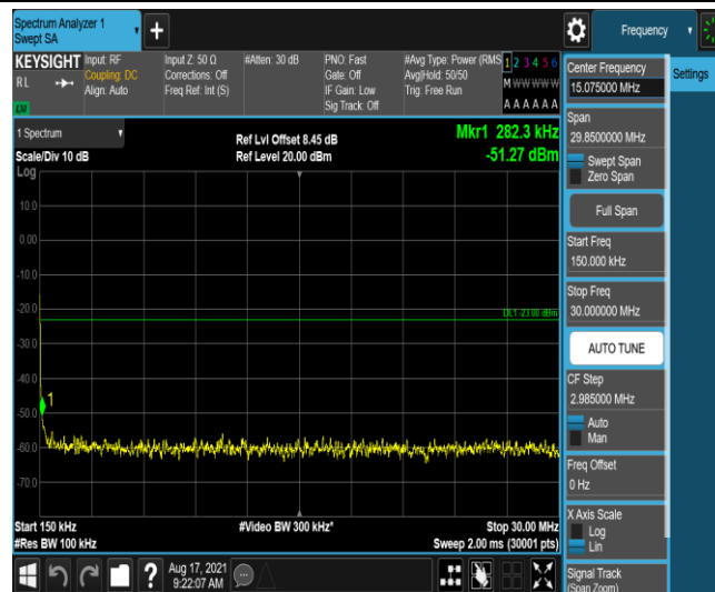
Band26-3MHz-16QAM-27025-1-0-High-0.15-30--51.27-PASS
