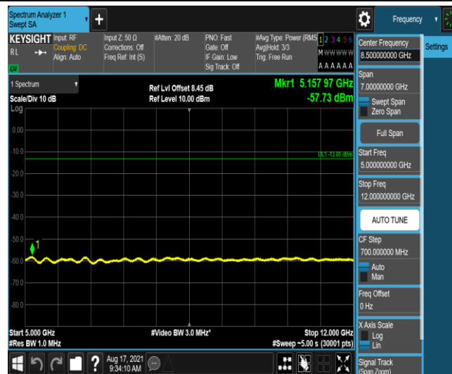
Band26-5MHz-QPSK-27015-1-0-High-5000-12000--57.73-PASS
