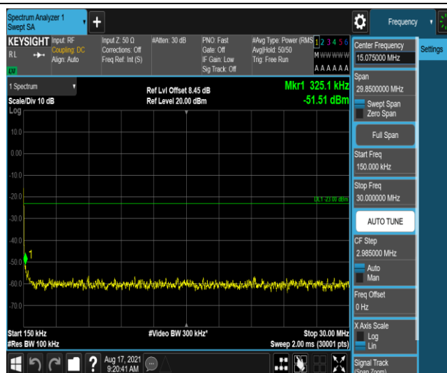
Band26-3MHz-QPSK-27025-1-0-High-0.15-30--51.51-PASS
