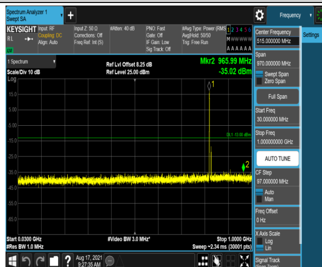
Band26-5MHz-QPSK-26815-1-0-Low-30-1000--35.02-PASS
