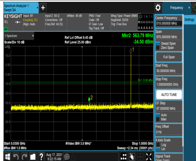
Band26-3MHz-16QAM-27025-1-0-High-30-1000--34.5-PASS
