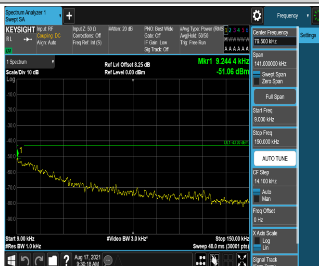
Band26-5MHz-QPSK-26915-1-0-Low-0.009-0.15--51.06-PASS
