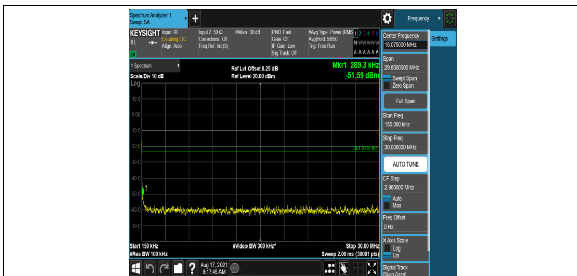
Band26-3MHz-QPSK-26915-1-0-Low-0.15-30--51.59-PASS
