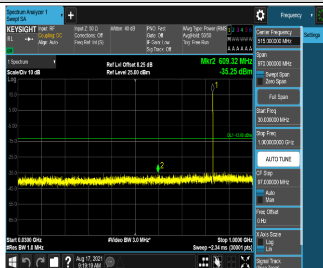
Band26-3MHz-16QAM-26915-1-0-Low-30-1000--35.25-PASS
