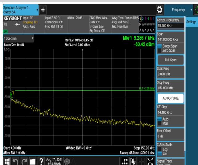
Band26-5MHz-16QAM-27015-1-0-High-0.009-0.15--50.42-PASS
