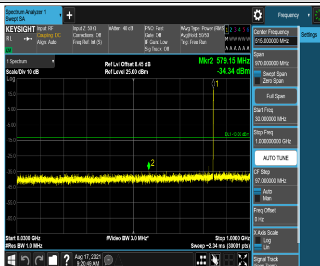
Band26-3MHz-QPSK-27025-1-0-High-30-1000--34.34-PASS
