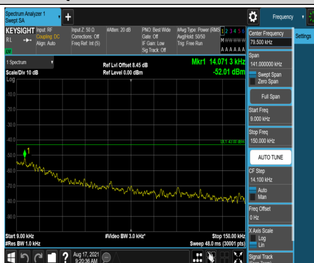
Band26-3MHz-QPSK-27025-1-0-High-0.009-0.15--52.01-PASS
