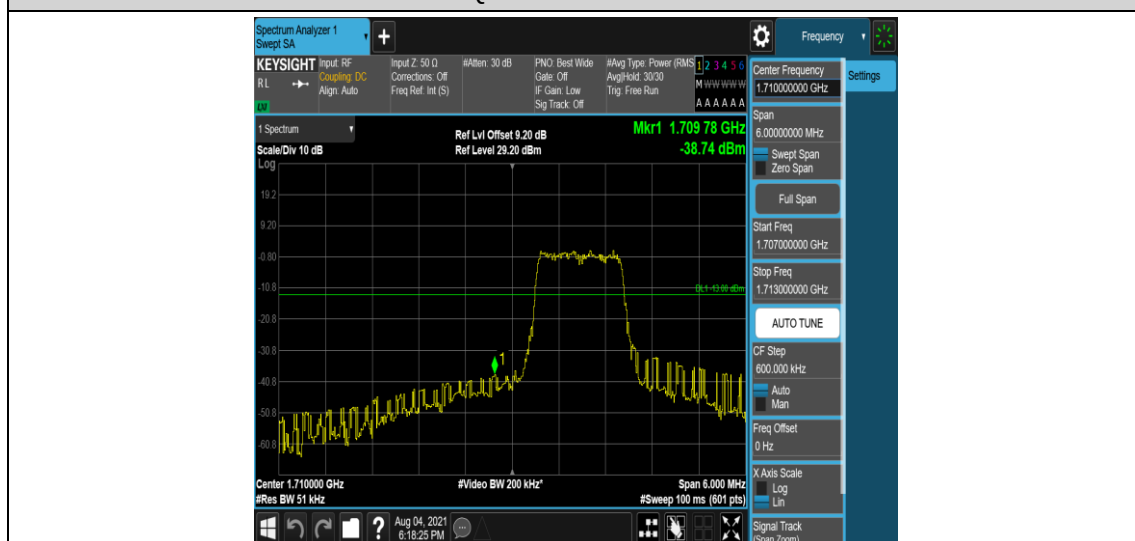
Band4-3MHz-16QAM-19965-6-0-Low--38.74-PASS
