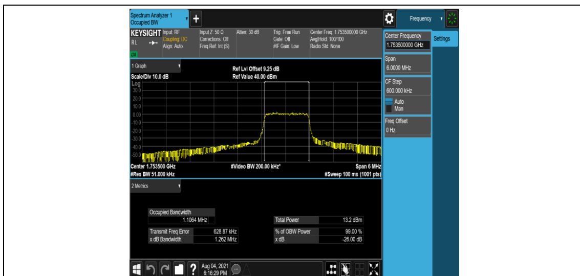
Band4-3MHz-16QAM-20385-6-0-High-1.1064-1.262-PASS
