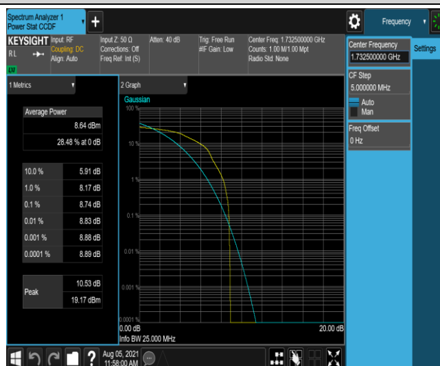
Band4-20MHz-16QAM-20175-1-0-Low-8.74-&lt;=13-PASS
