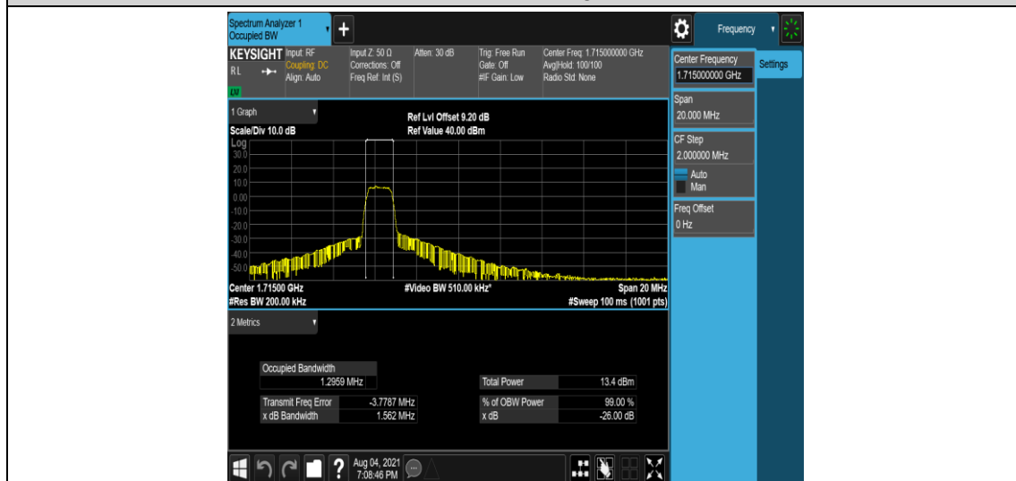
Band4-10MHz-QPSK-20000-6-0-Low-1.2959-1.562-PASS
