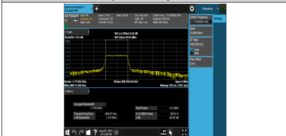
Band4-3MHz-QPSK-19965-6-0-Low-1.1163-1.315-PASS
