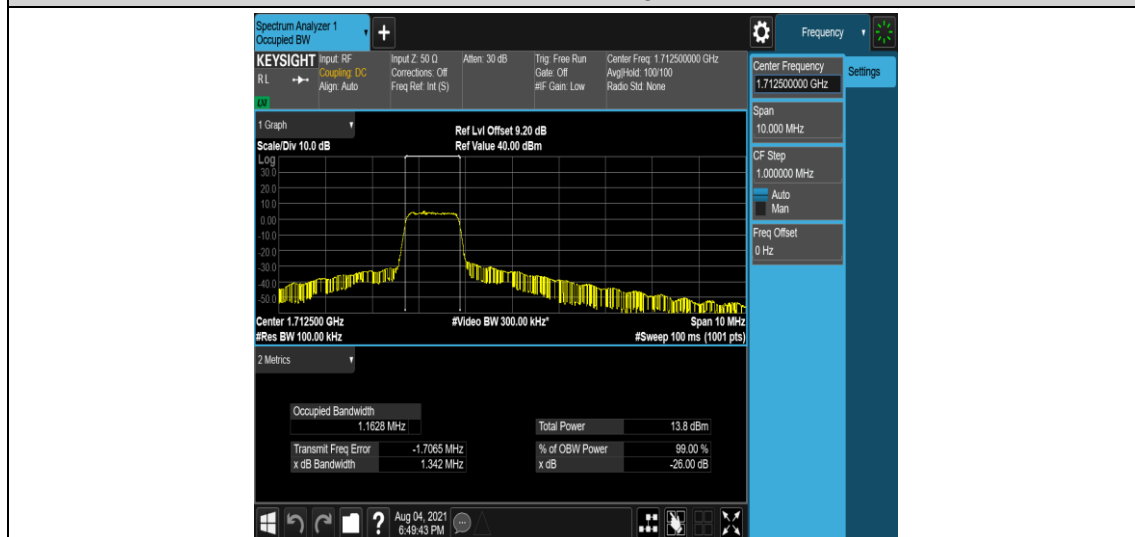
Band4-5MHz-16QAM-19975-6-0-Low-1.1628-1.342-PASS
