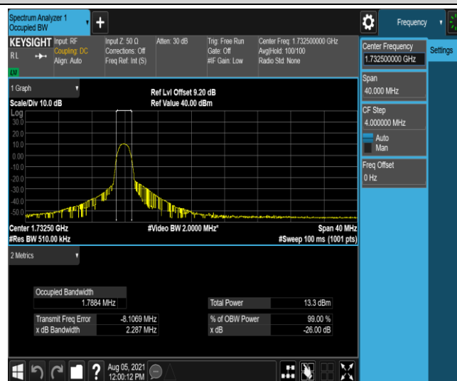
Band4-20MHz-16QAM-20175-6-0-Low-1.7884-2.287-PASS
