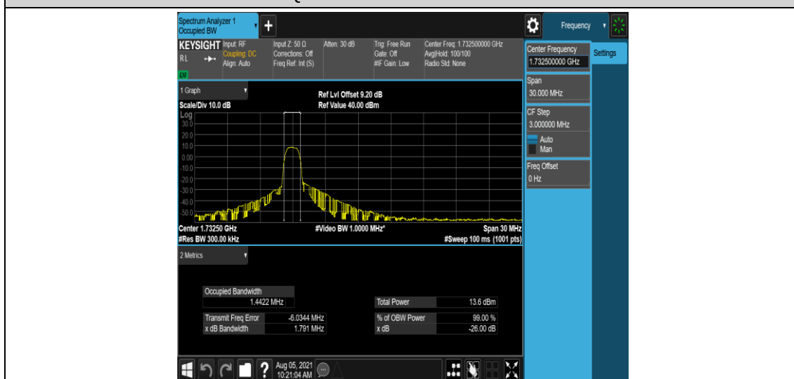
Band4-15MHz-QPSK-20175-6-0-Low-1.4422-1.791-PASS
