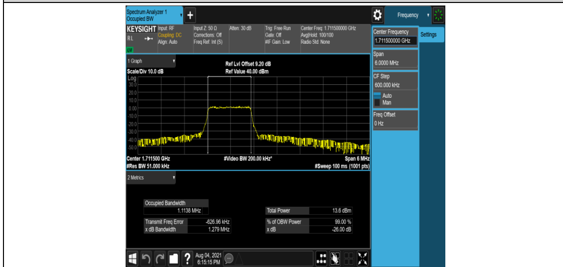
Band4-3MHz-16QAM-19965-6-0-Low-1.1138-1.279-PASS
