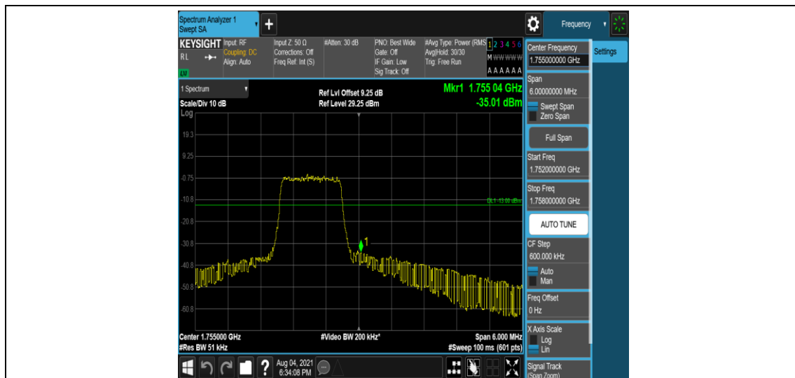
Band4-3MHz-QPSK-20385-6-0-High--35.01-PASS
