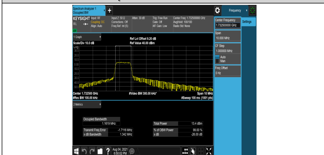
Band4-5MHz-QPSK-20175-6-0-Low-1.1619-1.342-PASS
