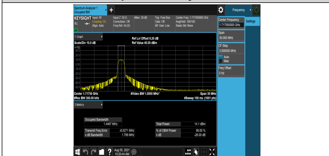
Band4-15MHz-16QAM-20025-6-0-Low-1.4467-1.795-PASS
