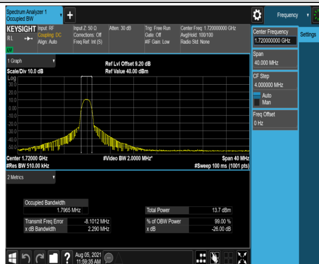
Band4-20MHz-16QAM-20050-6-0-Low-1.7965-2.290-PASS
