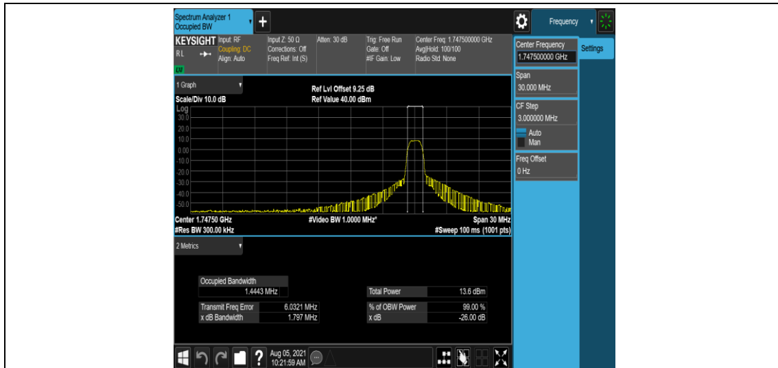
Band4-15MHz-16QAM-20325-6-0-High-1.4443-1.797-PASS
