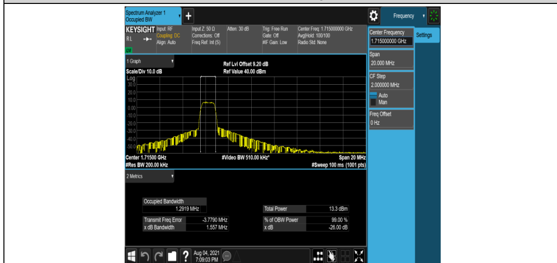
Band4-10MHz-16QAM-20000-6-0-Low-1.2919-1.557-PASS
