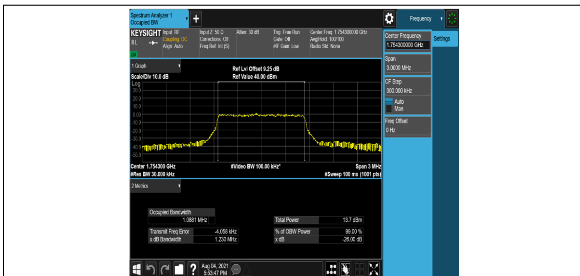
Band4-1.4MHz-16QAM-20393-6-0-High-1.0881-1.230-PASS
