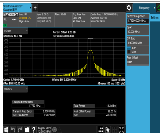
Band4-20MHz-QPSK-20300-6-0-High-1.7753-2.287-PASS
