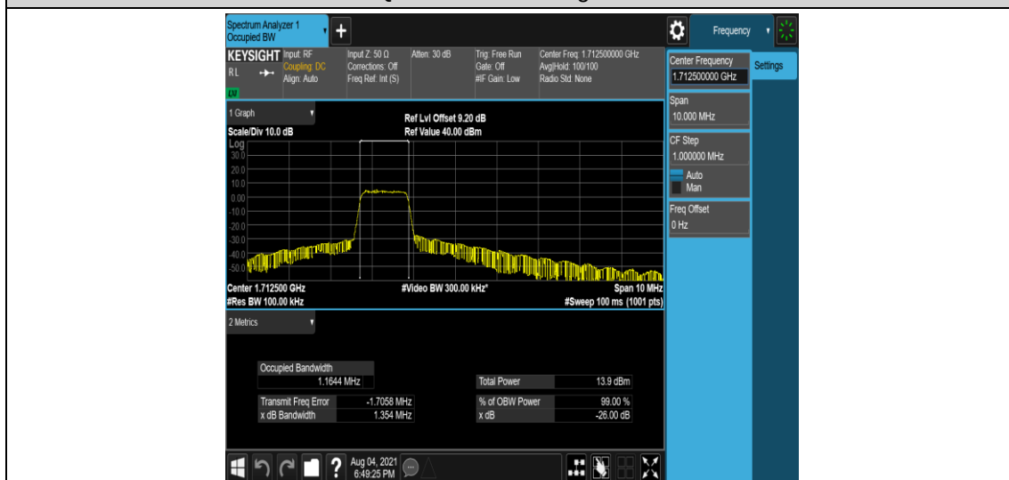
Band4-5MHz-QPSK-19975-6-0-Low-1.1644-1.354-PASS
