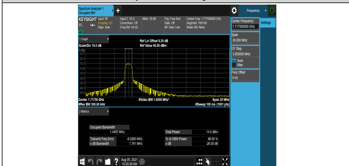
Band4-15MHz-QPSK-20025-6-0-Low-1.4497-1.791-PASS
