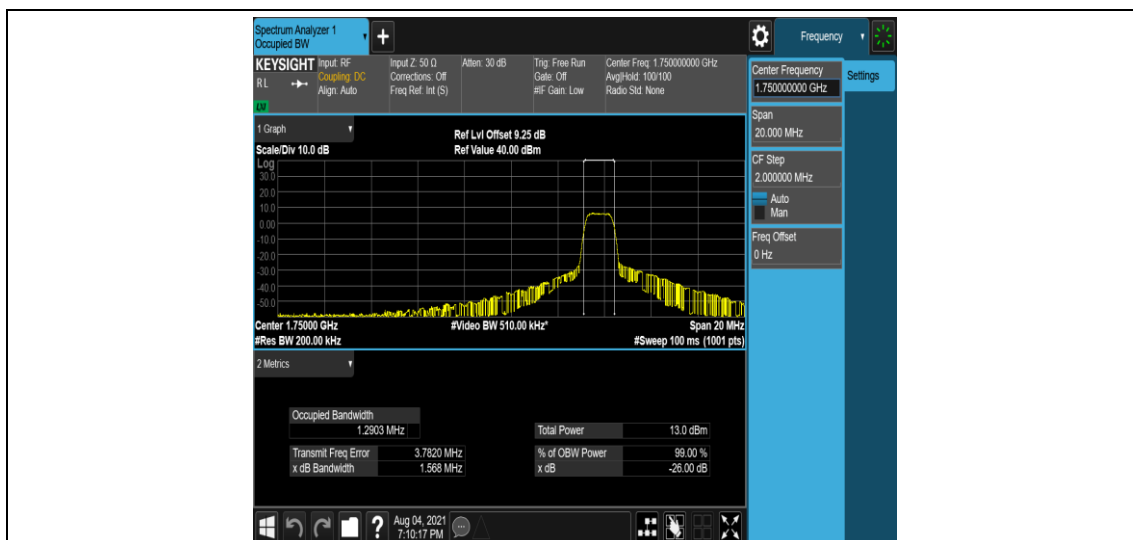
Band4-10MHz-16QAM-20350-6-0-High-1.2903-1.568-PASS
