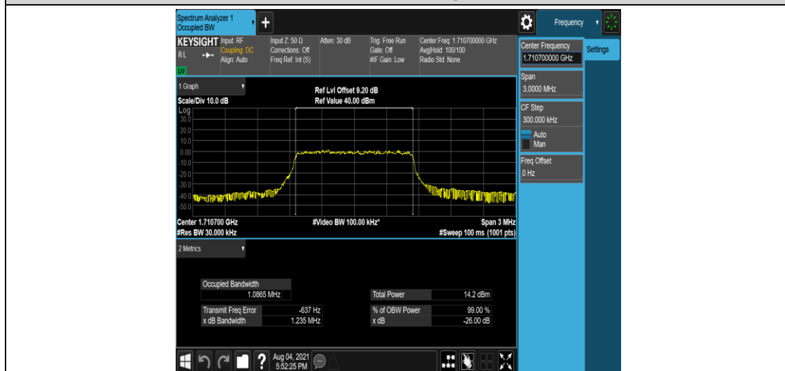
Band4-1.4MHz-16QAM-19957-6-0-Low-1.0865-1.235-PASS
