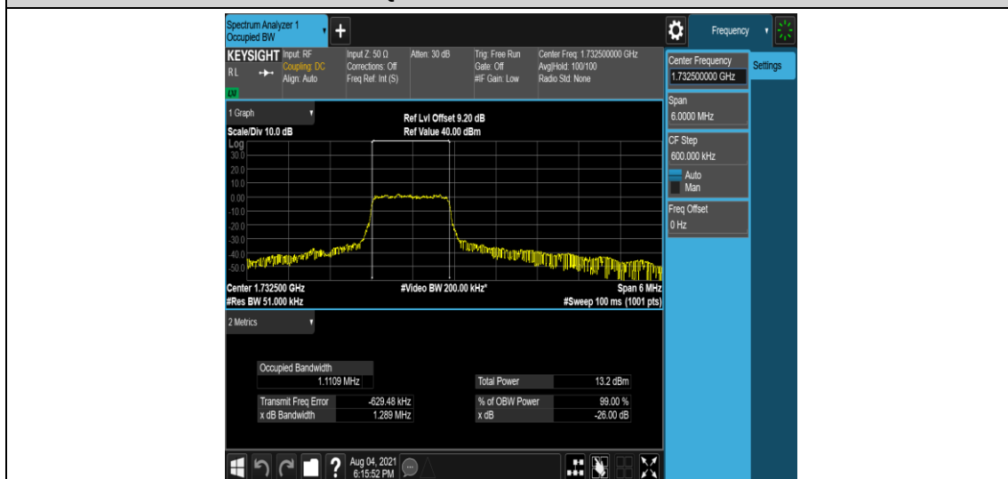
Band4-3MHz-16QAM-20175-6-0-Low-1.1109-1.289-PASS
