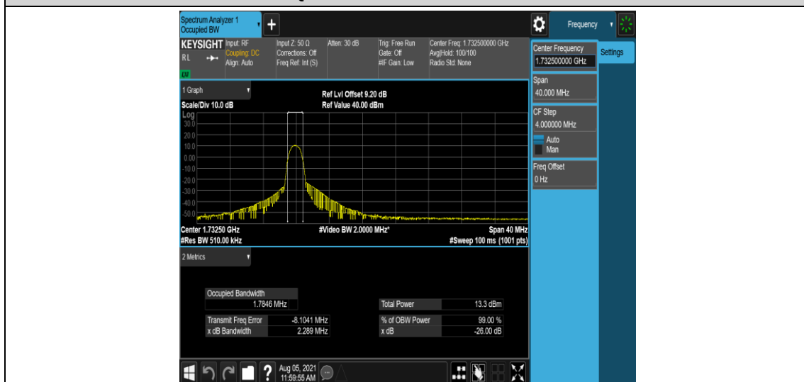
Band4-20MHz-QPSK-20175-6-0-Low-1.7846-2.289-PASS
