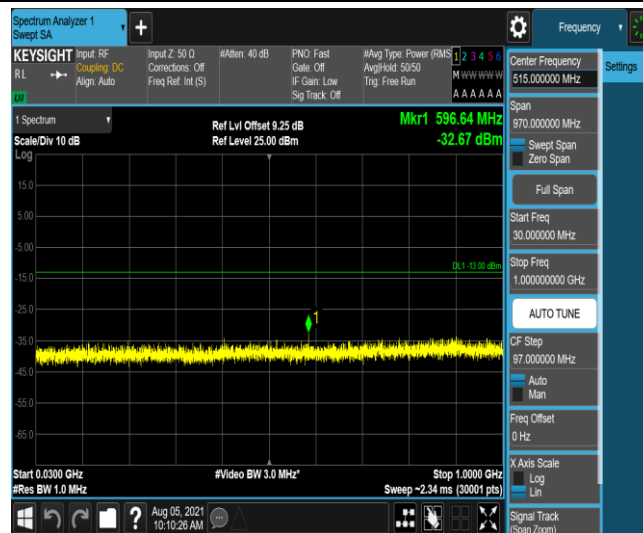
Band4-10MHz-QPSK-20350-1-0-High-30-1000--32.68-PASS
