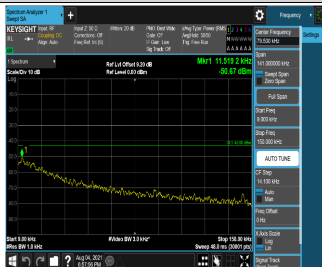
Band4-5MHz-16QAM-20175-1-0-Low-0.009-0.15--50.67-PASS
