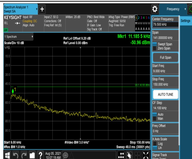
Band4-10MHz-QPSK-20175-1-0-Low-0.009-0.15--50.96-PASS
