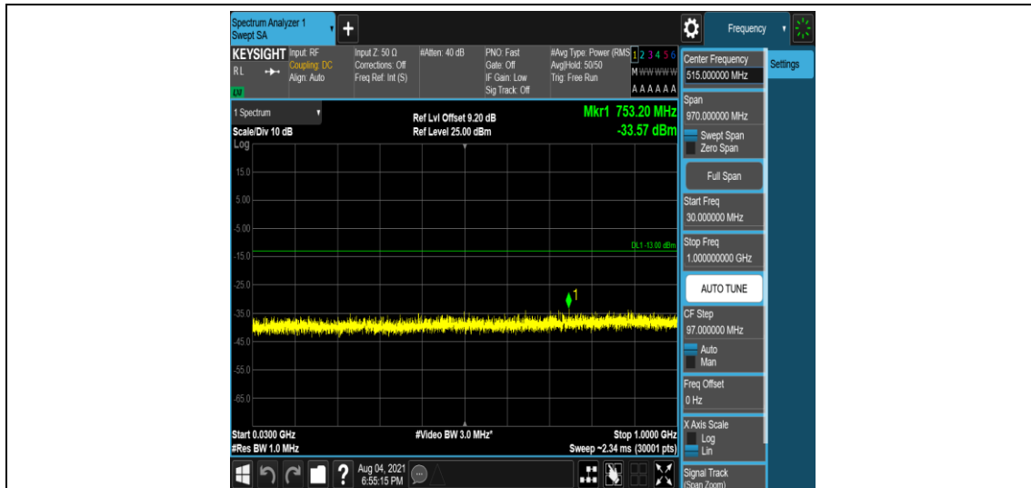
Band4-5MHz-16QAM-19975-1-0-Low-30-1000--33.57-PASS
