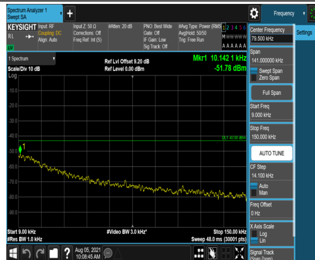
Band4-10MHz-16QAM-20175-1-0-Low-0.009-0.15--51.78-PASS
