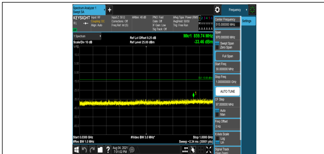
Band4-5MHz-16QAM-20375-1-0-High-30-1000--33.46-PASS
