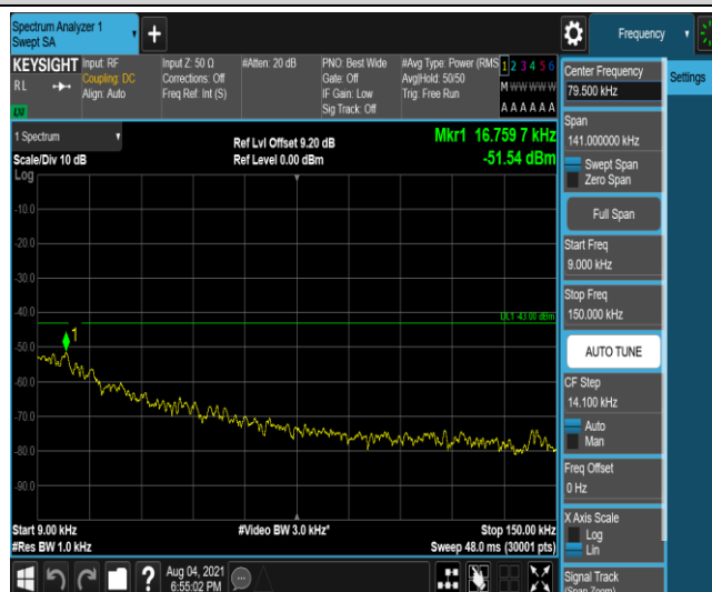
Band4-5MHz-16QAM-19975-1-0-Low-0.009-0.15--51.54-PASS
