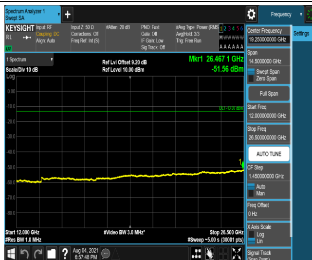
Band4-5MHz-QPSK-20175-1-0-Low-12000-26500--51.56-PASS
