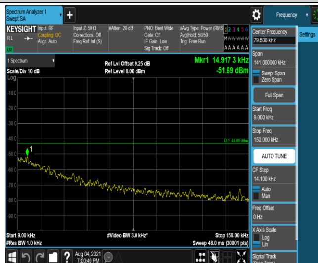
Band4-5MHz-16QAM-20375-1-0-High-0.009-0.15--51.69-PASS
