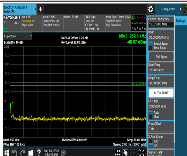
Band4-5MHz-QPSK-20375-1-0-High-0.15-30--48.07-PASS
