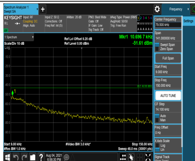
Band4-5MHz-QPSK-20175-1-0-Low-0.009-0.15--51.61-PASS
