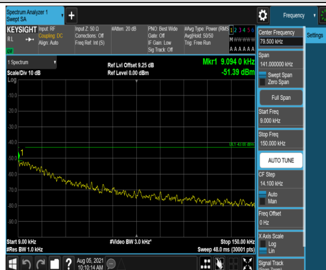
Band4-10MHz-QPSK-20350-1-0-High-0.009-0.15--51.39-PASS
