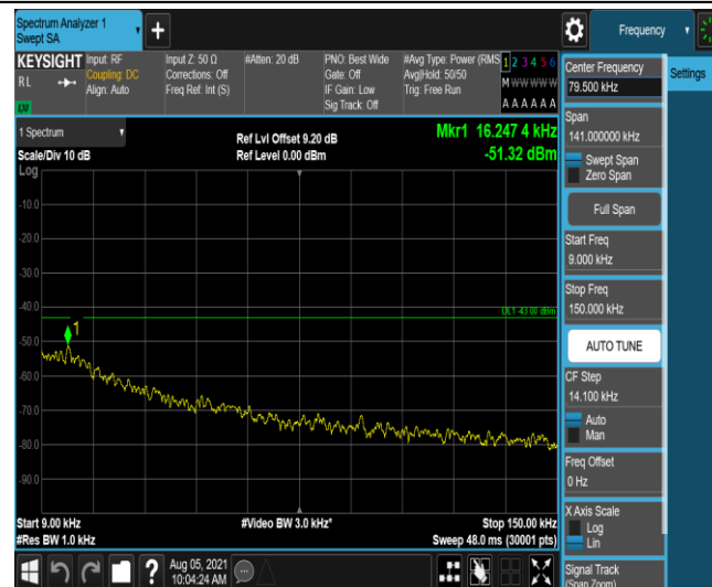
Band4-10MHz-QPSK-20000-1-0-Low-0.009-0.15--51.32-PASS
