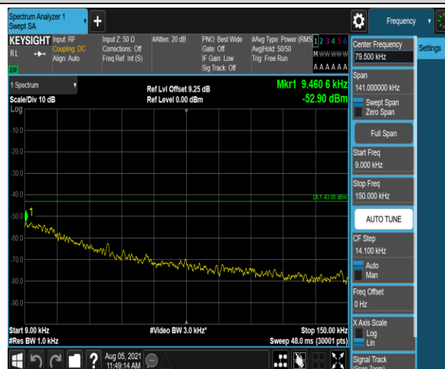
Band4-15MHz-16QAM-20325-1-0-High-0.009-0.15--52.9-PASS
