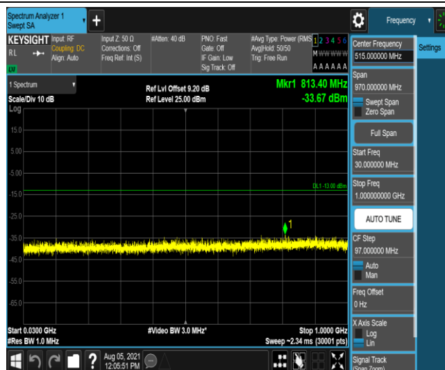
Band4-20MHz-QPSK-20175-1-0-Low-30-1000--33.67-PASS
