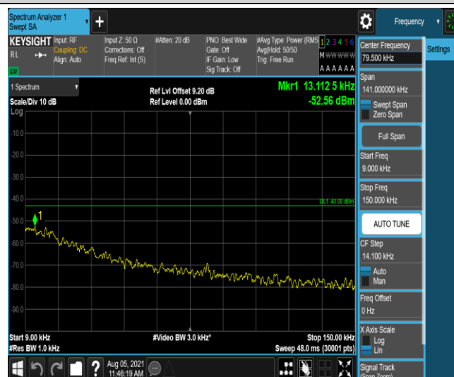
Band4-15MHz-16QAM-20175-1-0-Low-0.009-0.15--52.56-PASS
