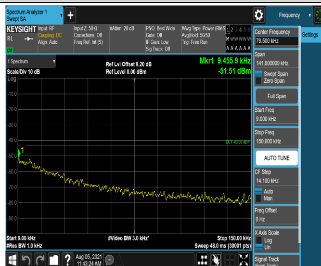
Band4-15MHz-16QAM-20025-1-0-Low-0.009-0.15--51.51-PASS
