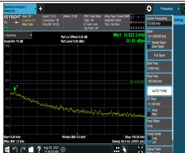
Band4-15MHz-QPSK-20175-1-0-Low-0.009-0.15--51.81-PASS
