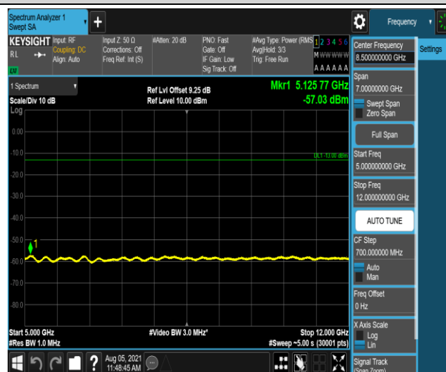
Band4-15MHz-QPSK-20325-1-0-High-5000-12000--57.03-PASS
