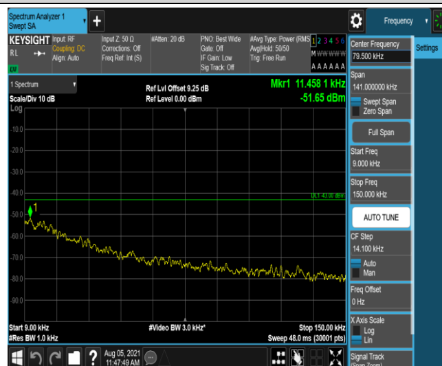
Band4-15MHz-QPSK-20325-1-0-High-0.009-0.15--51.65-PASS
