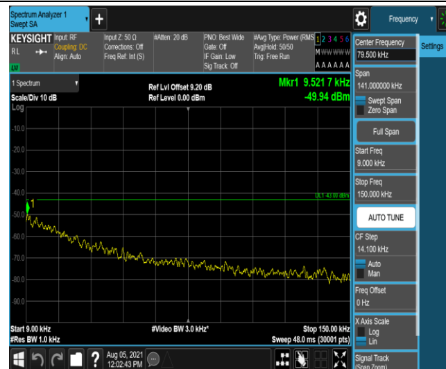
Band4-20MHz-QPSK-20050-1-0-Low-0.009-0.15--49.94-PASS
