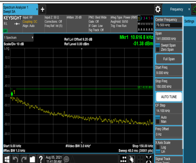
Band4-15MHz-QPSK-20025-1-0-Low-0.009-0.15--51.38-PASS
