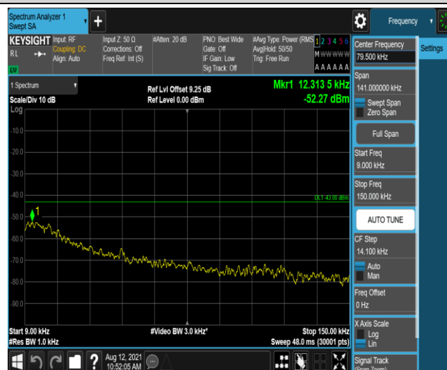
Band66-10MHz-QPSK-132322-1-0-Low-0.009-0.15--52.27-PASS
