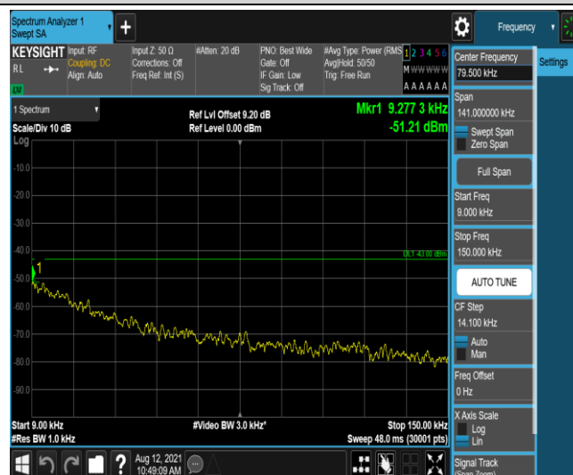
Band66-10MHz-QPSK-132022-1-0-Low-0.009-0.15--51.21-PASS
