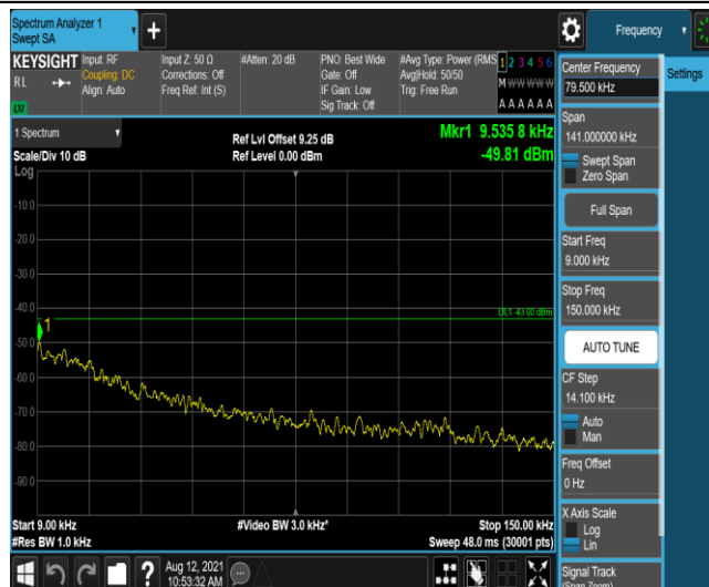
Band66-10MHz-16QAM-132322-1-0-Low-0.009-0.15--49.81-PASS
