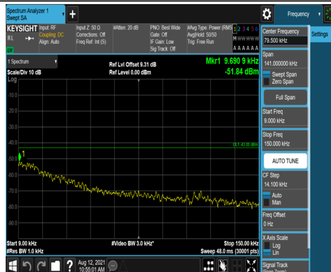
Band66-10MHz-QPSK-132622-1-0-High-0.009-0.15--51.84-PASS
