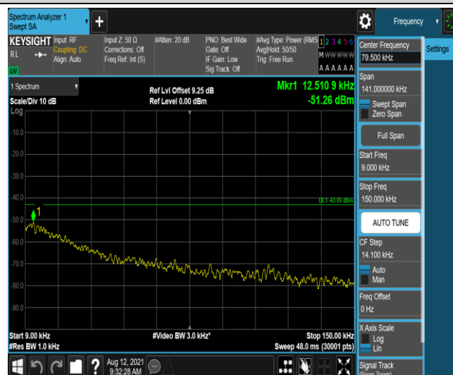
Band66-5MHz-16QAM-132322-1-0-Low-0.009-0.15--51.26-PASS
