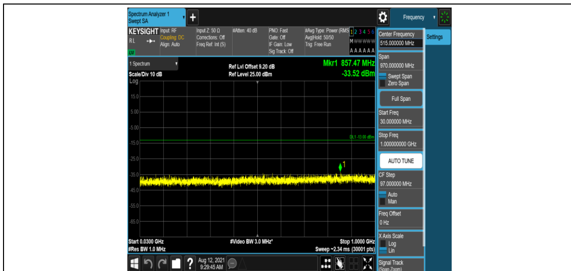
Band66-5MHz-16QAM-131997-1-0-Low-30-1000--33.52-PASS
