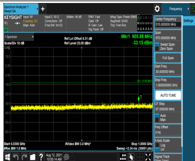
Band66-10MHz-QPSK-132622-1-0-High-30-1000--33.15-PASS
