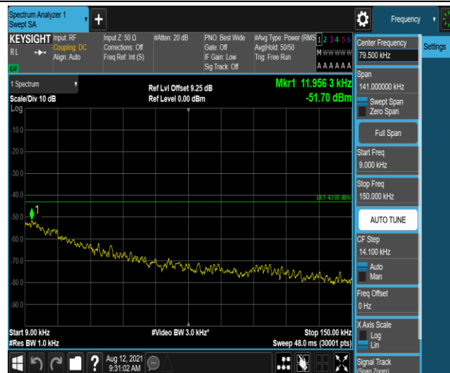
Band66-5MHz-QPSK-132322-1-0-Low-0.009-0.15--51.7-PASS
