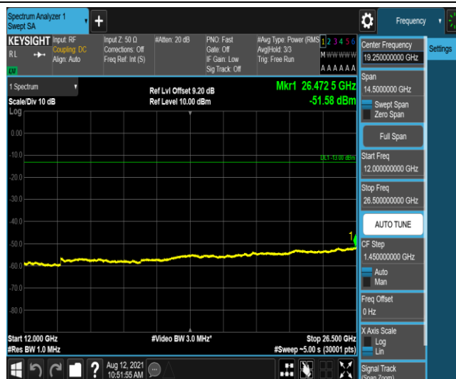
Band66-10MHz-16QAM-132022-1-0-Low-12000-26500--51.58-PASS
