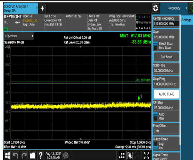
Band66-5MHz-QPSK-131997-1-0-Low-30-1000--33.83-PASS
