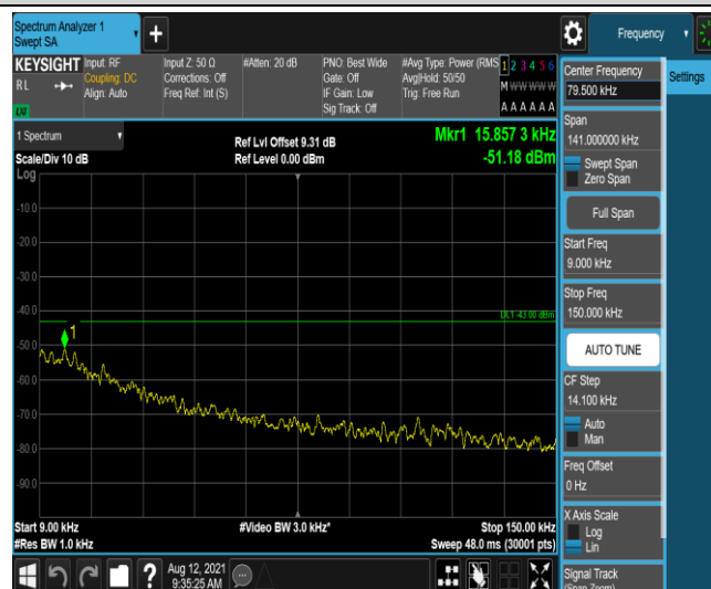
Band66-5MHz-16QAM-132647-1-0-High-0.009-0.15--51.18-PASS
