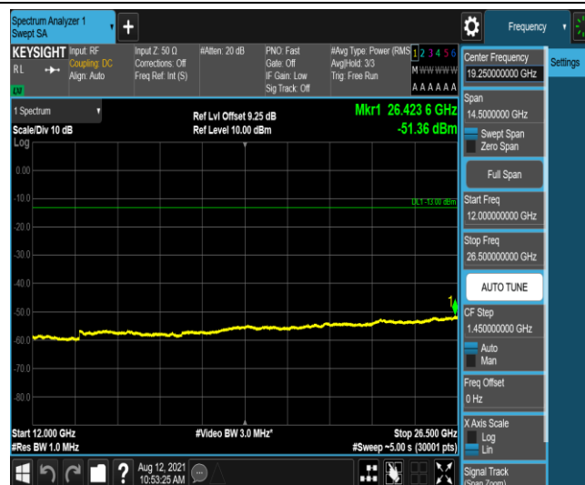
Band66-10MHz-QPSK-132322-1-0-Low-12000-26500--51.36-PASS
