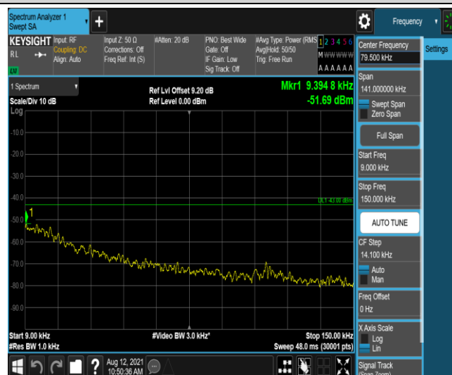
Band66-10MHz-16QAM-132022-1-0-Low-0.009-0.15--51.7-PASS
