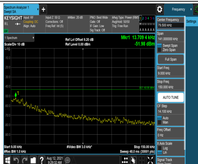
Band66-5MHz-16QAM-131997-1-0-Low-0.009-0.15--51.98-PASS
