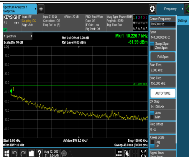
Band66-15MHz-QPSK-132047-1-0-Low-0.009-0.15--51.99-PASS
