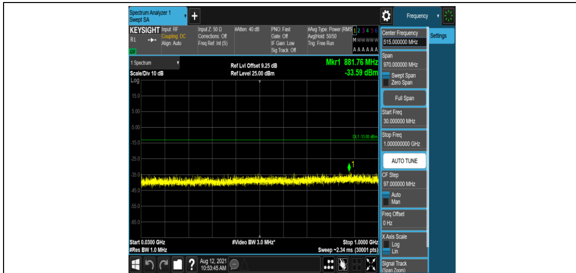
Band66-10MHz-16QAM-132322-1-0-Low-30-1000--33.59-PASS
