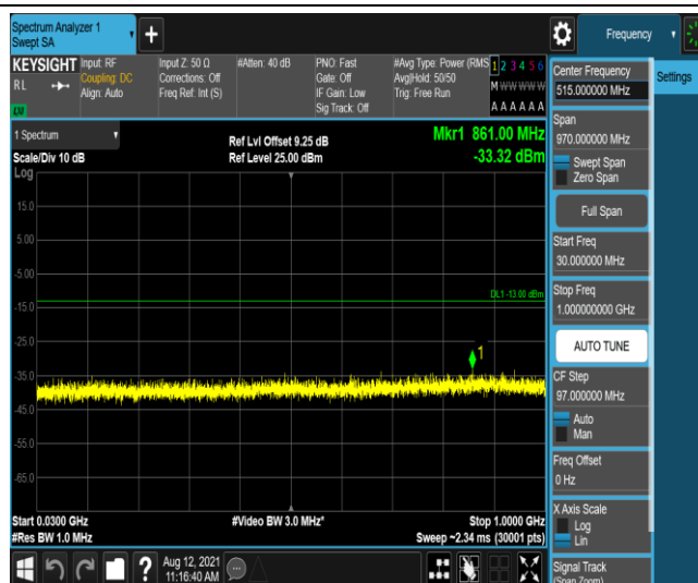
Band66-15MHz-QPSK-132322-1-0-Low-30-1000--33.32-PASS
