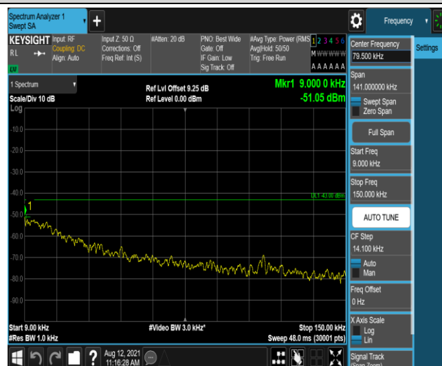
Band66-15MHz-QPSK-132322-1-0-Low-0.009-0.15--51.05-PASS
