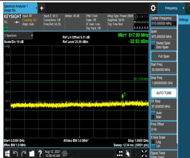
Band66-10MHz-16QAM-132622-1-0-High-30-1000--32.93-PASS
