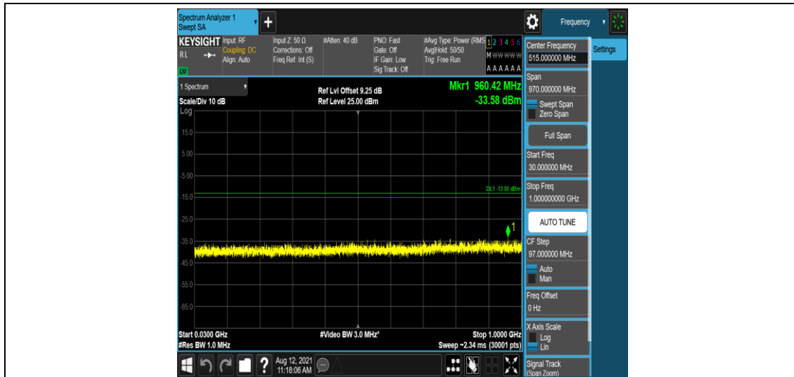
Band66-15MHz-16QAM-132322-1-0-Low-30-1000--33.58-PASS
