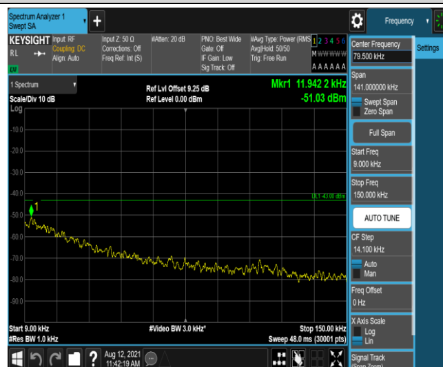
Band66-20MHz-QPSK-132322-1-0-Low-0.009-0.15--51.03-PASS
