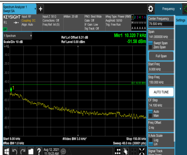
Band66-15MHz-QPSK-132597-1-0-High-0.009-0.15--51.58-PASS
