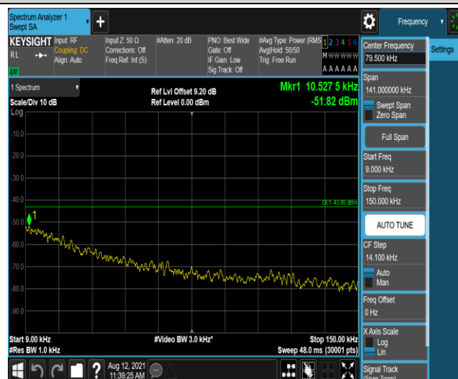
Band66-20MHz-QPSK-132072-1-0-Low-0.009-0.15--51.82-PASS
