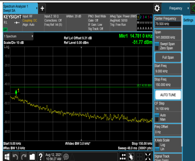
Band66-10MHz-16QAM-132622-1-0-High-0.009-0.15--51.77-PASS
