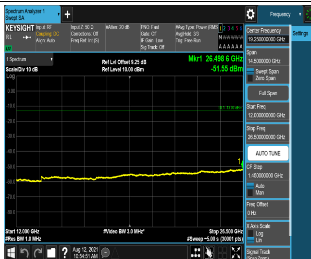
Band66-10MHz-16QAM-132322-1-0-Low-12000-26500--51.55-PASS
