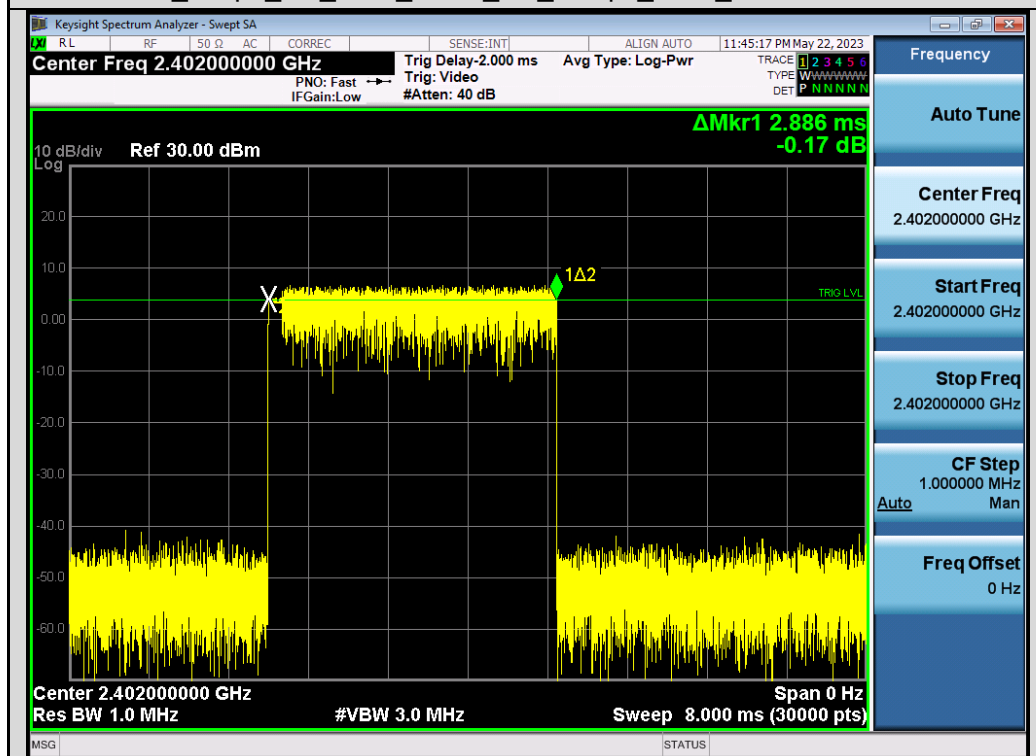
Test Graph BR HOP ANT1 NA 3Mbps 2402 Time per Burst 1 1 1 1 1 1 1 1 1 2 1 1 1 1 1 1 1 1 3 1 1 1 1 1 1 1 1 4 1 1 1 1 1 1 1 1 5 1 1 1 1 1 1 1 1 6 1 1 1 1 1 1 1 1 7 1 1 1 1 1 1 1 1 8 1 1 1 1 1 1 1 1 9 1 1 1 1 1 1 1 1 10 1 1 1 1 1 1 1 1 11 1 1 1 1 1 1 1 1 12 1 1 1 1 1 1 1 1 13 1 1 1 1 1 1 1 1 14 1 1 1 1 1 1 1 1 15 1 1 1 1 1 1 1 1 16 1 1 1 1 1 1 1 1 17 1 1 1 1 1 1 1 1 18 1 1 1 1 1 1 1 1 19 1 1 1 1 1 1 1 1 20 1 1 1 1 1 1 1 1 21 1 1 1 1 1 1 1 1 22 1 1 1 1 1 1 1 1 23 1 1 1 1 1 1 1 1 24 1 1 1 1 1 1 1 1 25 1 1 1 1 1 1 1 1 26 1 1 1 1 1 1 1 1 27 1 1 1 1 1 1 1 1 28 1 1 1 1 1 1 1 1 29 1 1 1 1 1 1 1 1 30 1 1 1 1 1 1 1 1 31 1 1 1 1 1 1 1 1 32 1 1 1 1 1 1 1 1 33 1 1 1 1 1 1 1 1 34 1 1 1 1 1 1 1 1 35 1 1 1 1 1 1 1 1 36 1 1 1 1 1 1 1 1 37 1 1 1 1 1 1 1 1 38 1 1 1 1 1 1 1 1 39 1 1 1 1 1 1 1 1 40 1 1 1 1 1 1 1 1 41 1 1 1 1 1 1 1 1 42 1 1 1 1 1 1 1 1 43 1 1 1 1 1 1 1 1 44 1 1 1 1 1 1 1 1 45 1 1 1 1 1 1 1 1 46 1 1 1 1 1 1 1 1 47 1 1 1 1 1 1 1 1 48 1 1 1 1 1 1 1 1 49 1 1 1 1 1 1 1 1 50 1 1 1 1 1 1 1 1 51 1 1 1 1 1 1 1 1 52 1 1 1 1 1 1 1 1 53 1 1 1 1 1 1 1 1 54 1 1 1 1 1 1 1 1 55 1 1 1 1 1 1 1 1 56 1 1 1 1 1 1 1 1 57 1 1 1 1</
