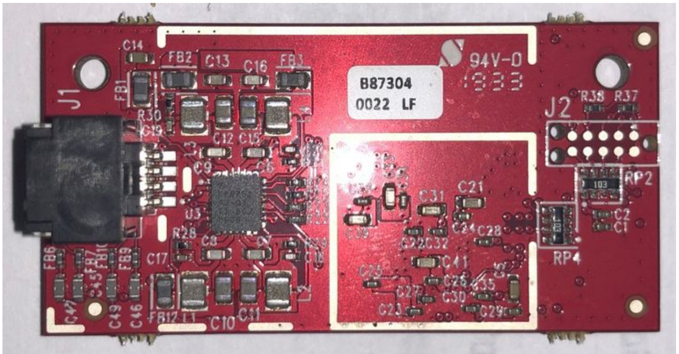
Figure 2. Patroness RADAR Module Back
