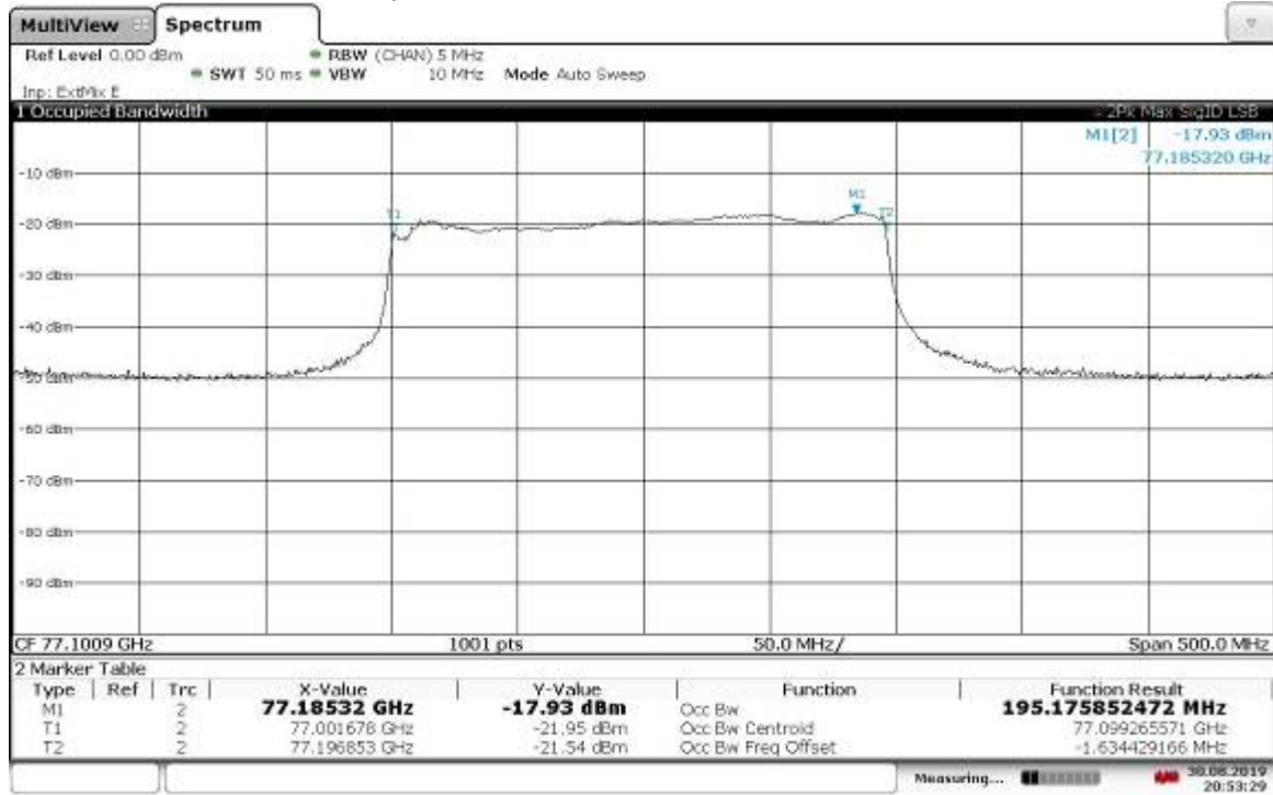
Occupied Bandwidth, Low Channel, 195.176 MHz
