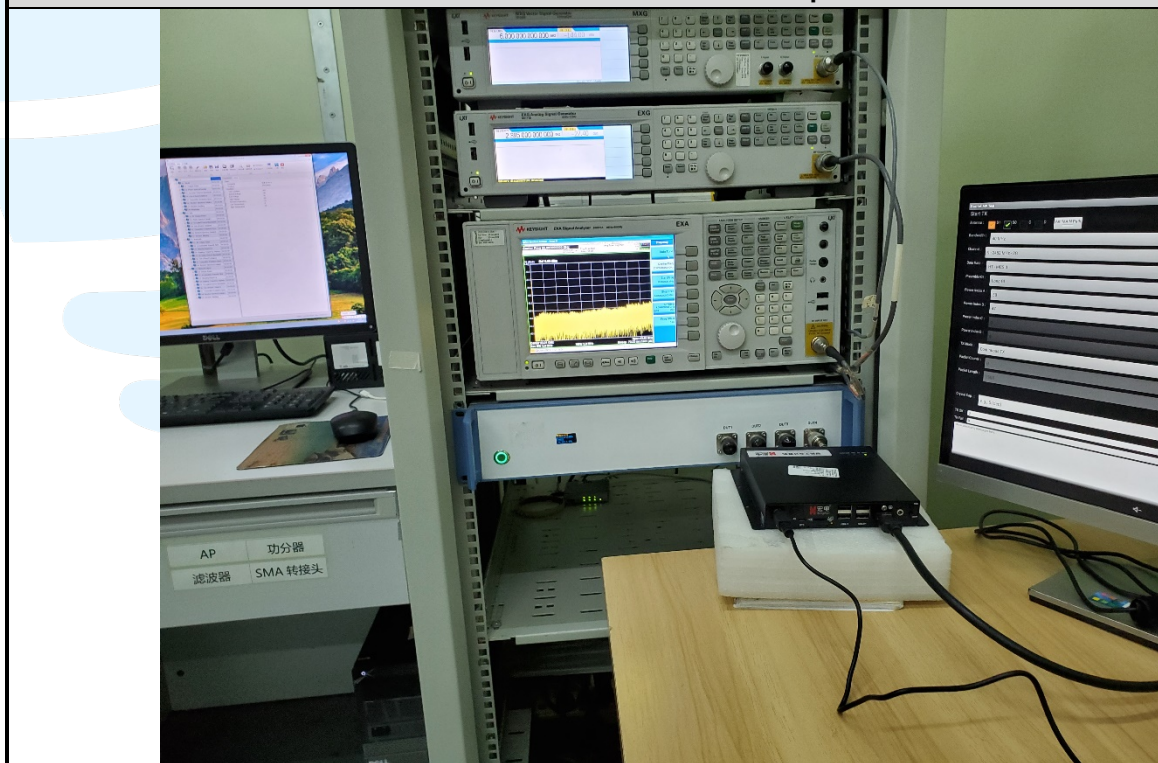
RF Conducted Test Setup
