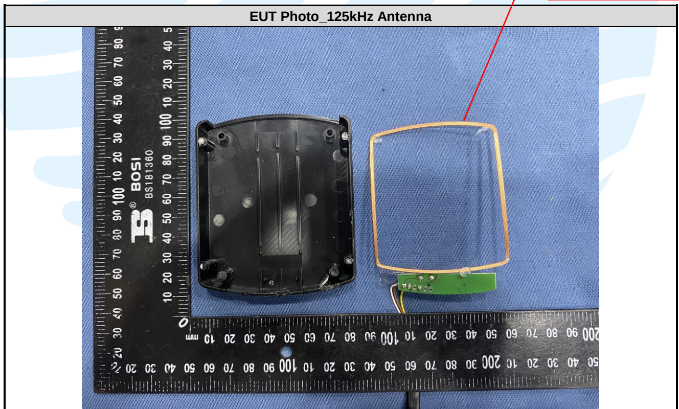
125 kHz Antenna
