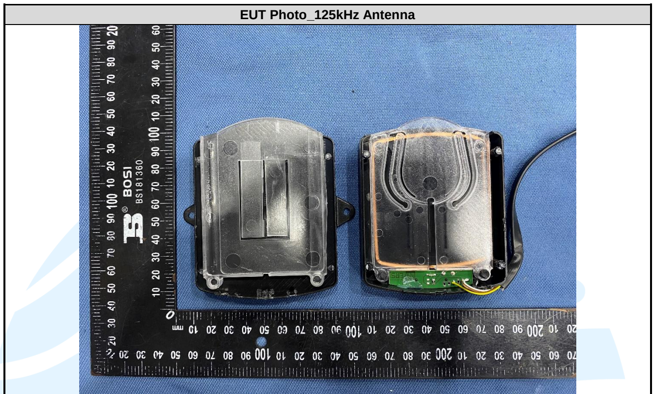
125 kHz Antenna
