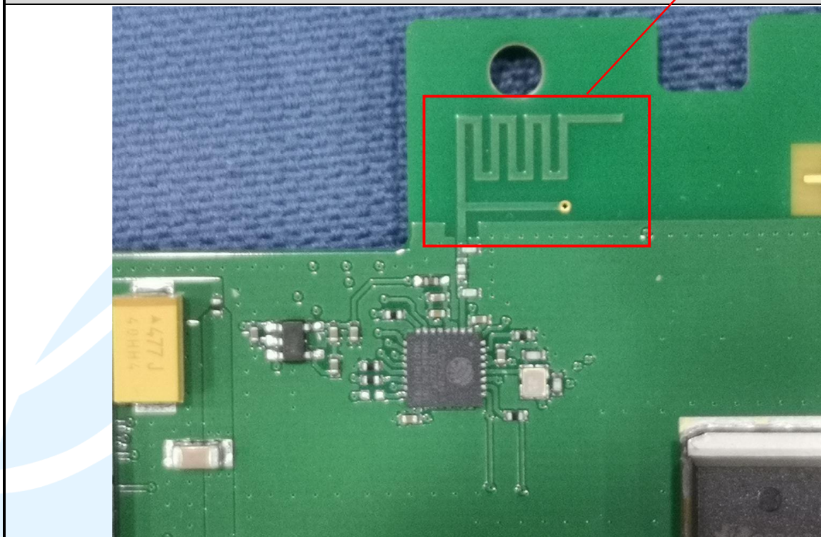
EUT Photo _ 2.4GHz Wi-Fi Receiver View
