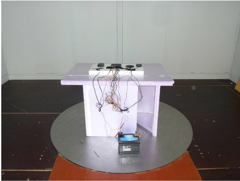
181948_5.JPG : Test setup final measurement from 30 to 1000 MHz OATS
