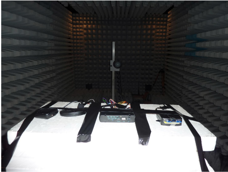
181948_3.JPG : Test setup final measurement from 1 to 14 GHz
