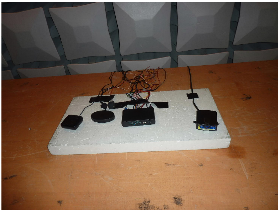
181948_2.JPG : Test setup preliminary measurement from 30 to 1000 MHz
