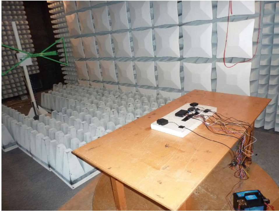
181948_1.JPG : Test setup preliminary measurement from 30 to 1000 MHz
