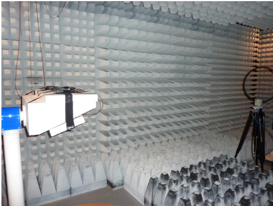
181948_6.JPG : Test setup preliminary measurement from 9 kHz to 30 MHz
