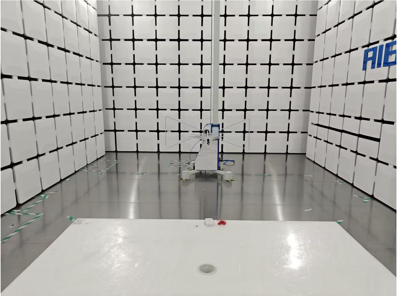
Radiated Spurious Emission Test View 1
