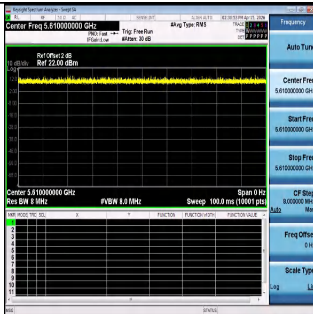
NTNV-11AC80MIMO-Ant1-5610
