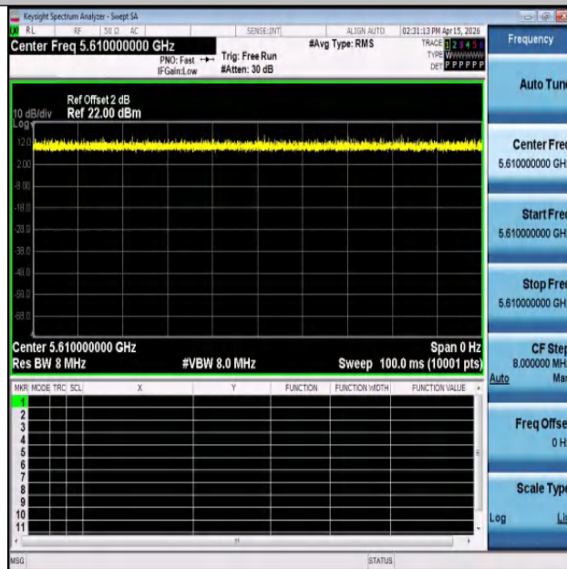
NTNV-11AC80MIMO-Ant2-5610
