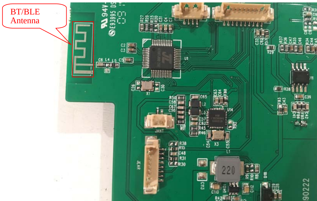
EUT – PCB-1 Chip View-2
