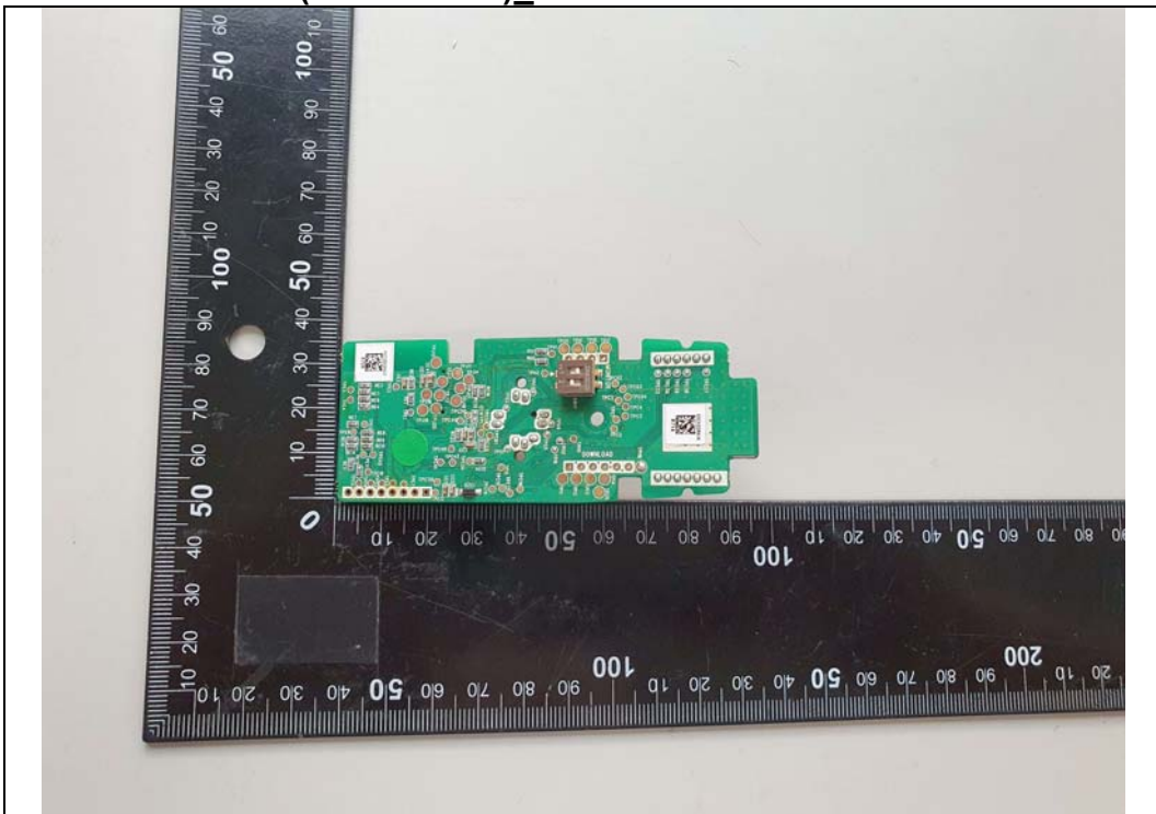
Derivative Model(EME501-SP) Main Board Rear
