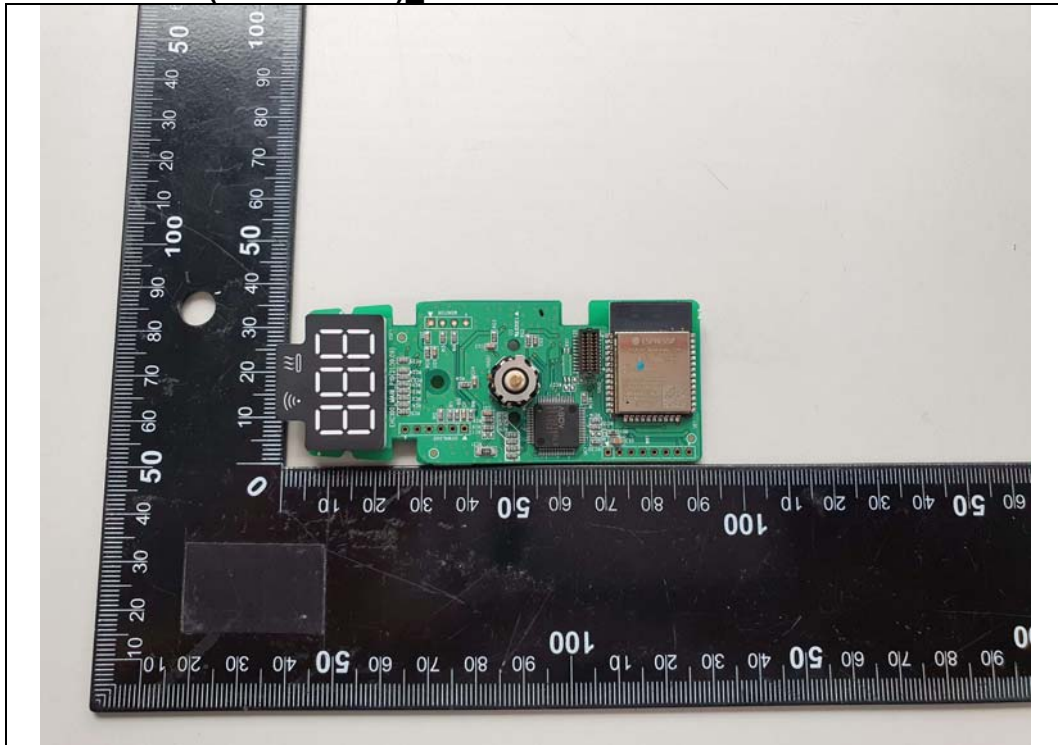
Basic Model(EME501-DP) Main Board Front
