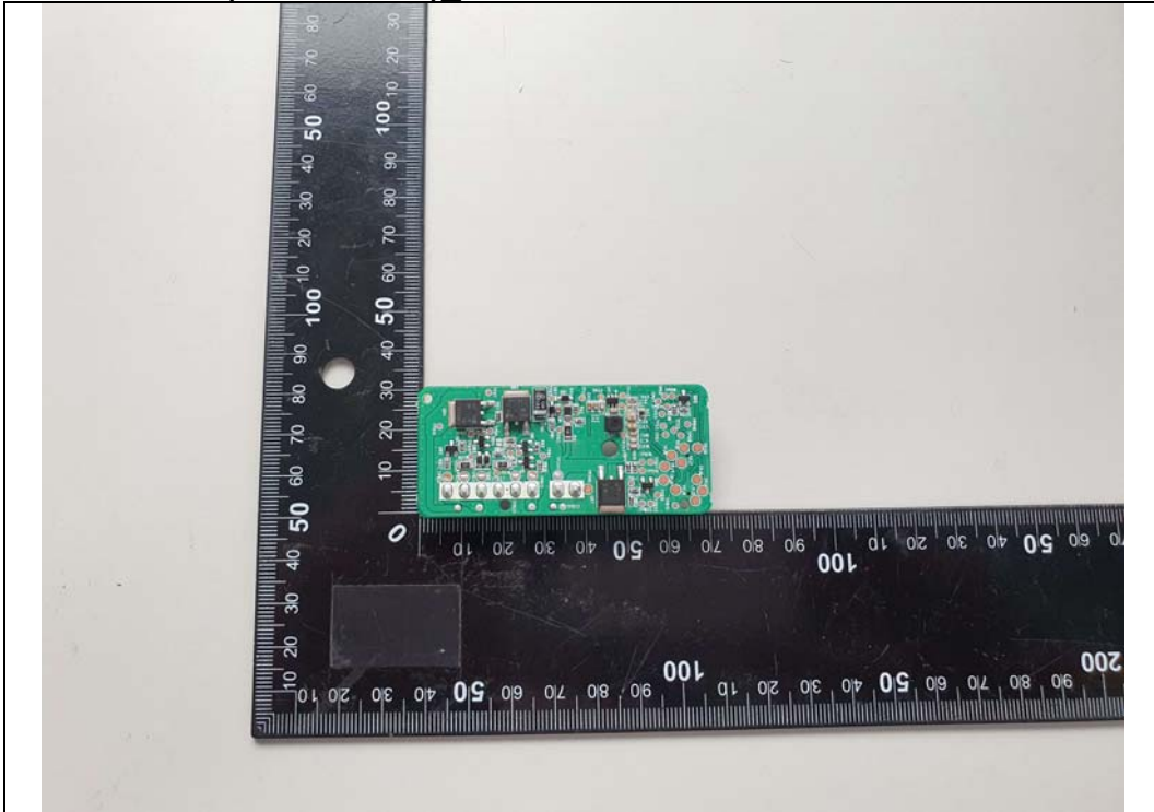
Basic Model(EME501-DP) Power Board Rear
