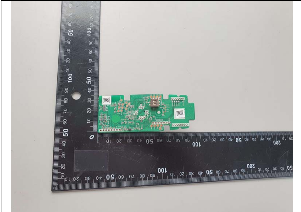
Basic Model(EME501-DP)_Main Board Rear
