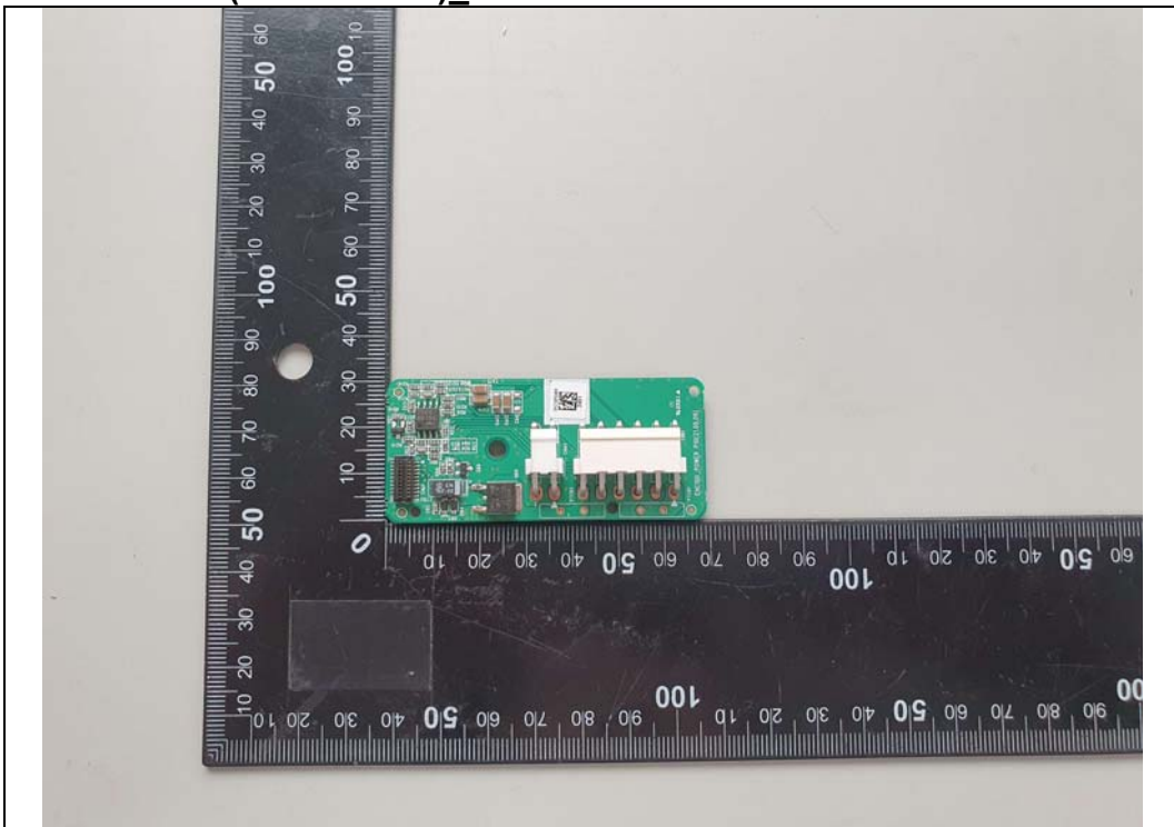
Basic Model(EME501-DP)_Power Board Front
