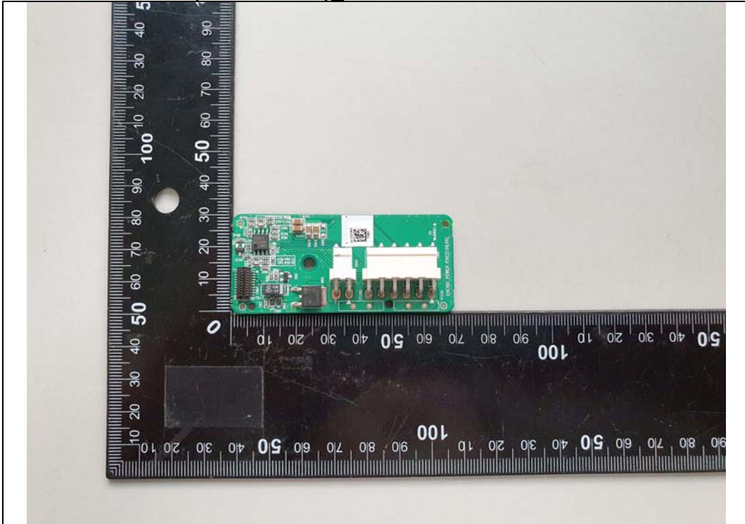
Derivative Model(EME501-SP)_Power Board Front
