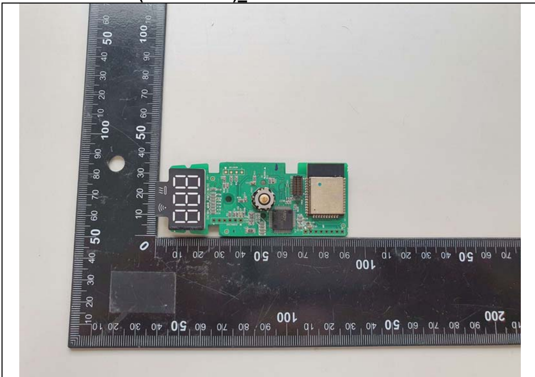
Derivative Model(EME501-SP) Main Board Front
