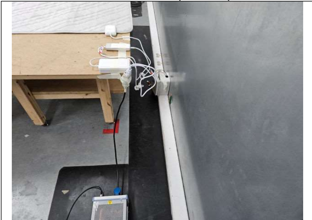
Conducted emission_Derivative model (EME511-SP) Rear
