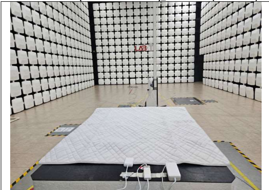
Radiated emission (30 MHz ~ 1 000 MHz) Basic model (EME511-KP) Rear
