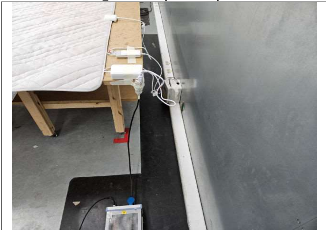
Conducted emission_Basic model (EME511-KP) Rear
