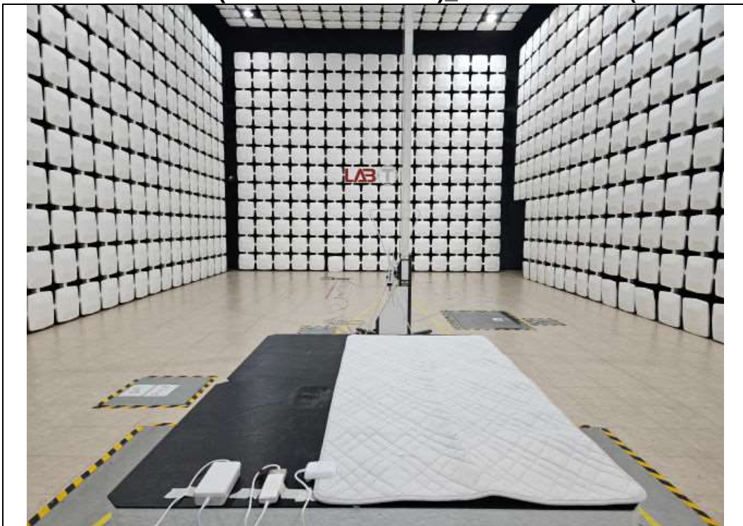
Radiated emission (30 MHz ~ 1 000 MHz) Derivative model (EME511-SP) Rear
