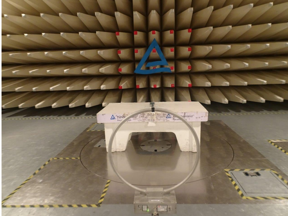
Photo 1 : 9KHz to 30MHz - Parallel polarization
