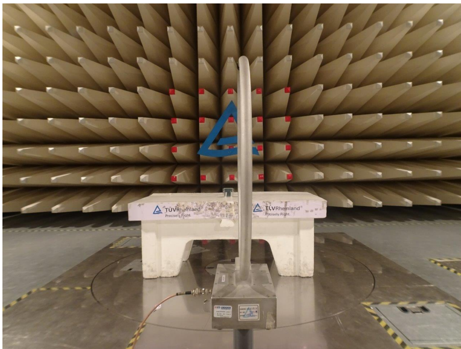
Photo 2: 9KHz to 30MHz - Perpendicular polarization
