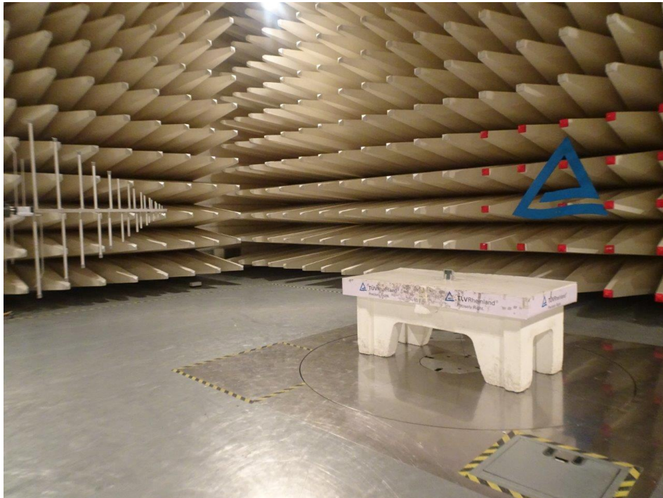
Photo 5: 200MHz to 1GHz - Vertical polarization
