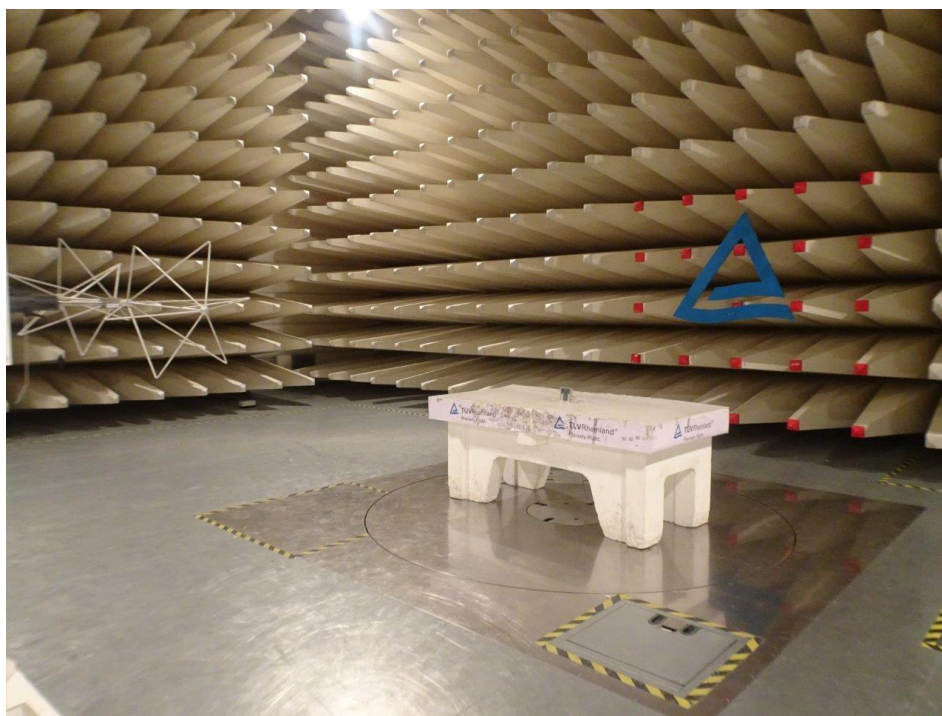
Photo 4: 30MHz to 200MHz - Horizontal polarization
