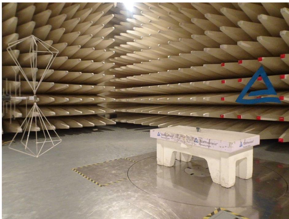
Photo 3: 30MHz to 200MHz - Vertical polarization
