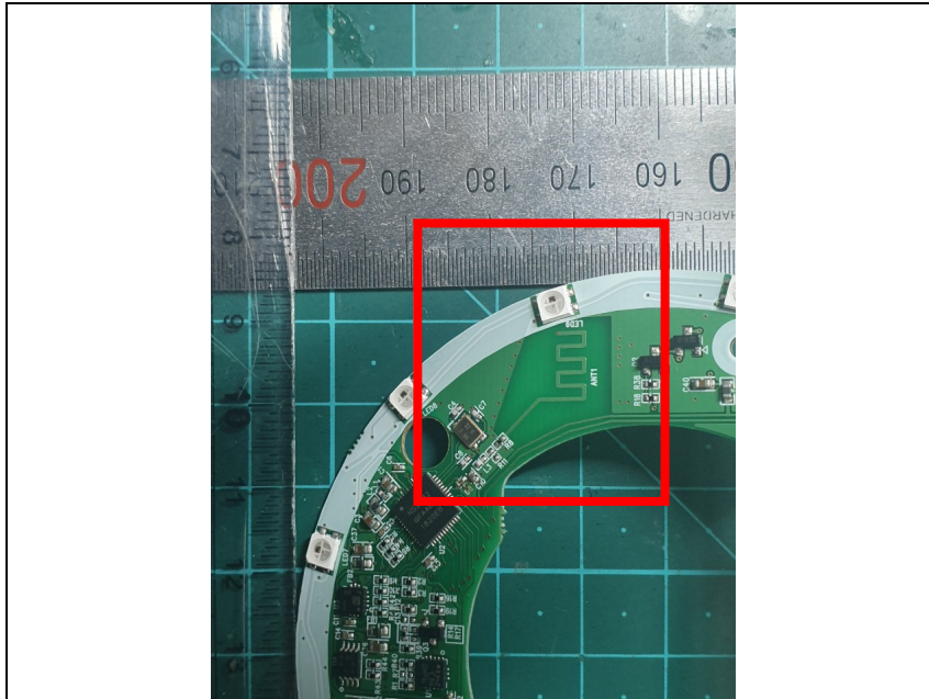
inside Port view of EUT
