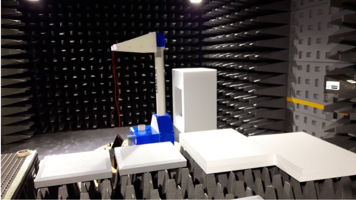
Test set up radiated emission 18 GHz – 26.5 GHz
