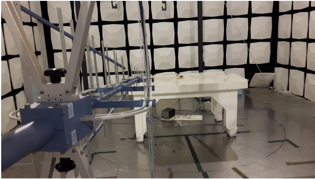
Test set up radiated emission 30 MHz – 1GHz
