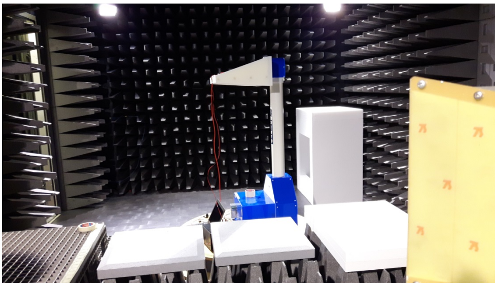
Test set up radiated emission 1GHz – 18 GHz
