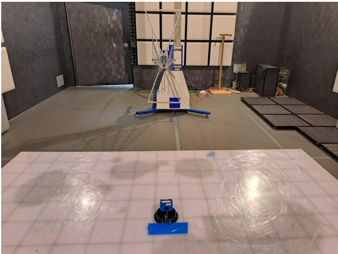
Figure 4: Spurious emission 30 MHz-1000 MHz
