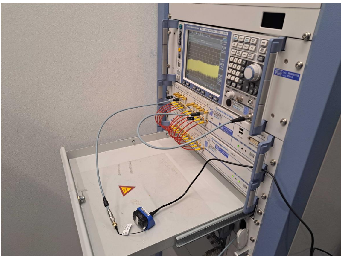
Figure 10: Conducted Spurious emission test setup
