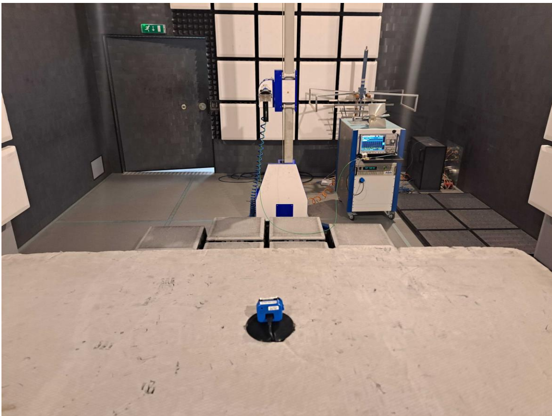
Figure 8: Spurious emission 18- 26 GHz
