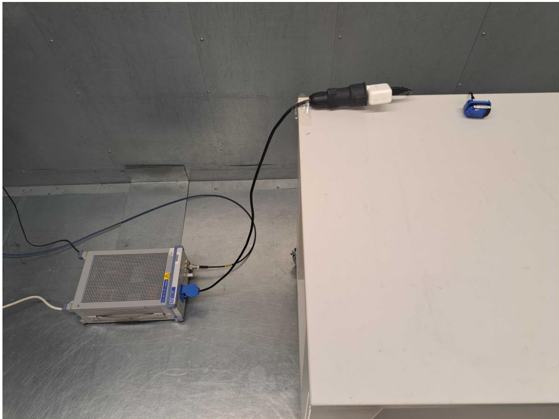
Figure 9: AC Conducted emission test setup
