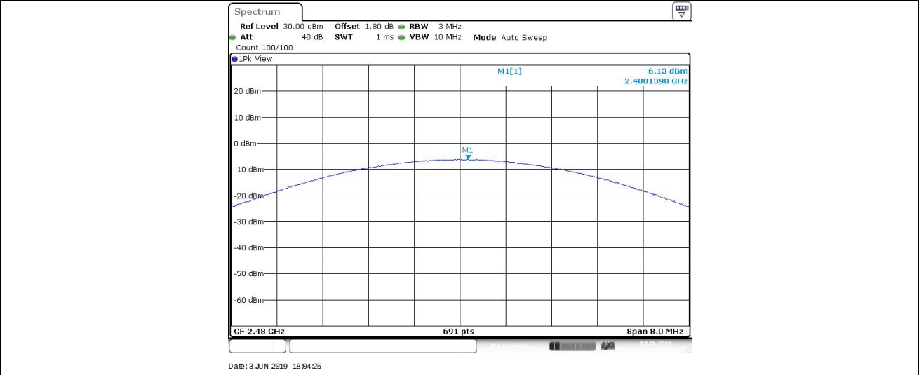
3DH5_Ant1_2480
